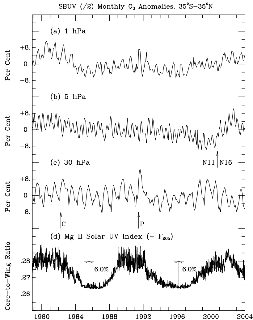
Figure 2. Time series of monthly zonal mean deviations of tropical (35°S to 35°N) SBUV(/2) ozone at (a) 1 hPa, (b) 5 hPa, and (c) 30 hPa over the 1979 to 2003 time period. (d) For comparison, time series of the daily Mg II solar UV index.
