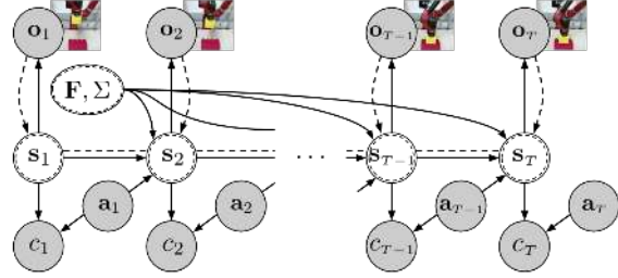
Figure 3 . Our generative model, in solid lines, and variational family and recognition network, in dashed lines. In practice, the observations we work with are RGB images, and we use convolutional neural networks for both the recognition and observation models. The distributions for each node are specified in Section 3 .
