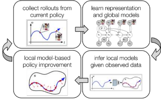
Figure 2. A high-level schematic of our method. We discuss the details of the model and inference procedure in Section 3 and Section 4. We then explain our algorithm in Section 5.
