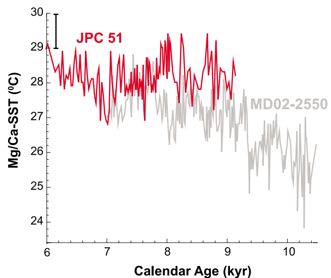
Figure 3. Comparison of the Mg/Ca-SST records from the Florida Straits (JPC 51 in red) and the northern Gulf of Mexico's Orca Basin (MD02-2550 in gray) [LoDico et al., 2006] calculated using the Mg/Ca-SST relationship in Anand et al. [2003]. The estimated \pm 1\sigma uncertainty on the JPC 51 SST record is shown by the black bar on the y axis. Because the Orca Basin SST record is also based on Mg/Ca ratios in G. ruber and has been calibrated using the same Mg/Ca-SST relationship [Anand et al., 2003], the estimated error on this record is assumed to be similar.
