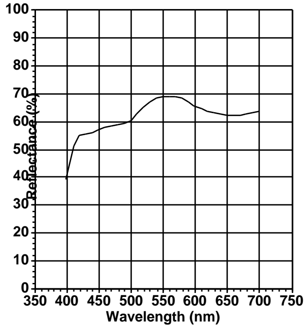
Figure 1. Venetian Blind Slat Hemispherical Spectral Reflectance
