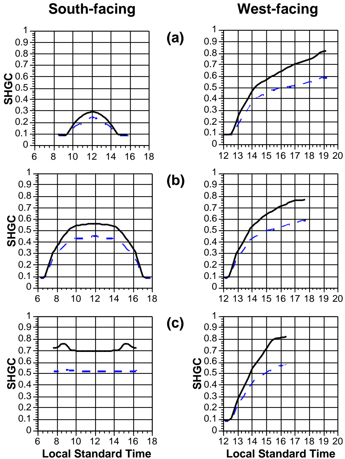
Figure 6. Effective SHGC as a function of time for clear double glazing with interior buff blind. For sun positions as would occur in Saint Louis, MO, the SHGC that would occur for a blind with horizontal slats (solid curves) or a 45° slat tilt (dashed curves) are shown for south-facing (left) and west-facing (right) orientations for (a) the summer solstice, (b) the spring/fall equinox, and (c) the winter solstice.
