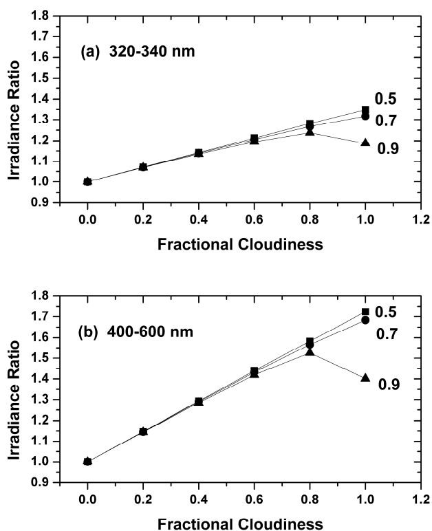
Fig. 9. Computed irradiance ratios as functions of fractional cloudiness for cloud albedos of A_c=0.5 , 0.7 and 0.9 . The solar disk is not obscured by clouds, and the ground albedo is A_G = 0.98 . (a) 320–340 nm wavelength band. (b) 400–600 nm wavelength band.
