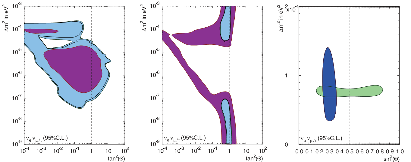
FIG. 15 (color). The left plot shows SK excluded areas. The purple region is SK-II and the light blue region is SK-I with SK-II. The black line shows SK-I only, and evidence of increased exclusion can be seen with the addition of SK-II data. The center plot shows SK allowed regions (same representative colors as the exclusion contours) with the ^8\text{B} flux constrained to the SNO total flux measurement. The hep flux is a free parameter. The right plot shows the SK-I and SK-II combined contour with SNO and radiochemical solar experimental data (blue contour). The green contour is the KamLAND electron antineutrino oscillation result.
