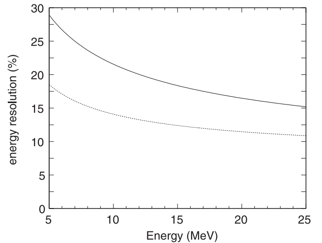
FIG. 5. Energy resolution as a function of total recoil electron energy of MC events. The dashed line is SK-I.
