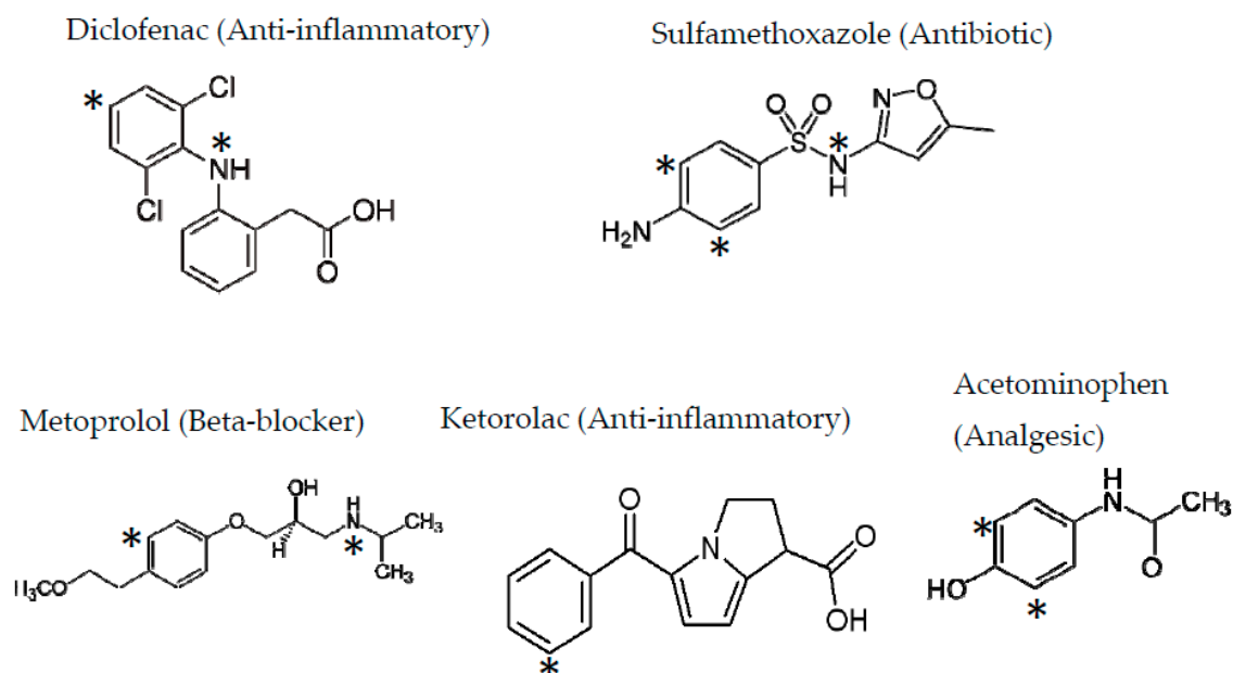
Figure 2. Examples of molecular structures of some pharmaceuticals usually found in urban wastewater. * Possible points of ozone attack.
