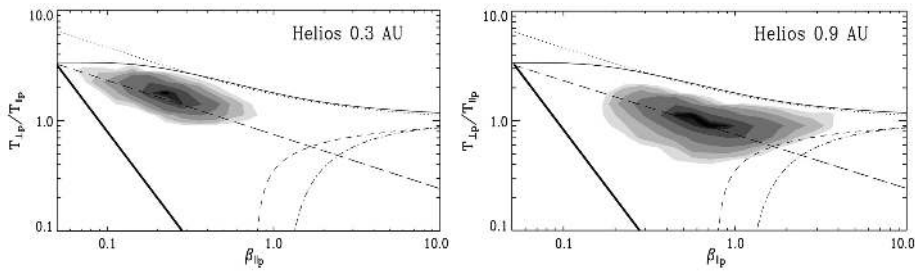
Figure 9. Histograms of the solar wind proton temperature anisotropy (ratio of perpendicular to parallel temperatures) versus the plasma pressure parallel to the field (parallel plasma beta) in the fast solar wind measured at two different radial distances by Helios. The dark line shows the decrease of anisotropy expected if the wind were expanding adiabatically without heating (dark continuous), and the actual distribution function contours with best fit of the run of anisotropy. Instability threshold conditions for the ion-cyclotron (solid), the mirror (dotted), the parallel (dashed) and oblique (dash-dotted) fire hose instabilities are also shown. Distribution functions display perpendicular heating and evolve towards marginal stability with distance from the Sun. Solar Orbiter will determine initial conditions for the perpendicular anisotropies and help determine the nature of the plasma-wave interactions responsible for this heating. (From Matteini et al. , 2007)
