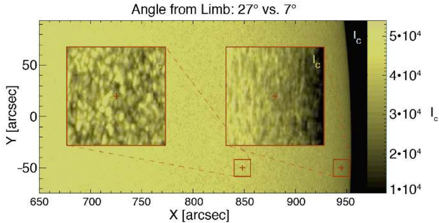
Figure 18. Comparison of solar granulation at the poles as viewed from 27^\circ , where the fine scale structure can be resolved with much higher fidelity than from ( 7^\circ ) inclination, obtained in the ecliptic plane twice a year. Hinode observations of the latter were used to obtain the first polar map of the vector magnetic field map (Tsuneta et al. , 2008). Solar Orbiter will characterize the properties and dynamics of the polar regions in detail, including magnetic fields, plasma flows, and temperatures.
