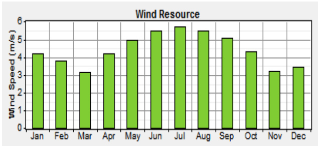
Figure 7. Bar graph showing wind resource
