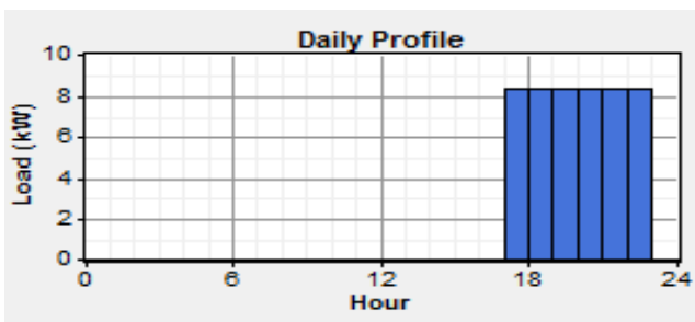
Figure 9. Bar graph showing daily load profile for NEC-TUM
