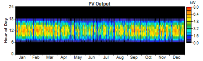
Figure 13. DMAP for solar PV
