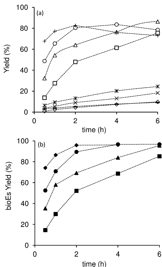
Fig. 7 Dependency of the yields of (a) 5EMF (+, \circ , \Delta , \square ) and EL (*, *, *, *), or (b) bioEs ( \blacklozenge , \bullet , \blacktriangle , \blacksquare ) on the time of the reaction of HMF in the presence of CST-0.1 ( \square , \diamond , \blacksquare ), CST-0.4 ( \Delta , - , \blacktriangle ) or CST-1 ( \circ , \times , \bullet ) at 110 °C, or in the presence of CST-1 at 140 °C (+, *, \blacklozenge ). Reaction conditions: [\text{HMF}]_0 = 0.33 \text{ M} ; catalyst loading = 10 \text{ g}_{\text{cat}} \text{ dm}^{-3} (the dashed lines are guides to the eye).
