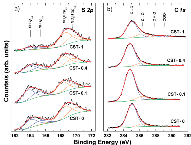
Fig. 4 Deconvoluted (a) S 2p and (b) C 1s X-ray photoelectron spectra of the CST- R composites.
