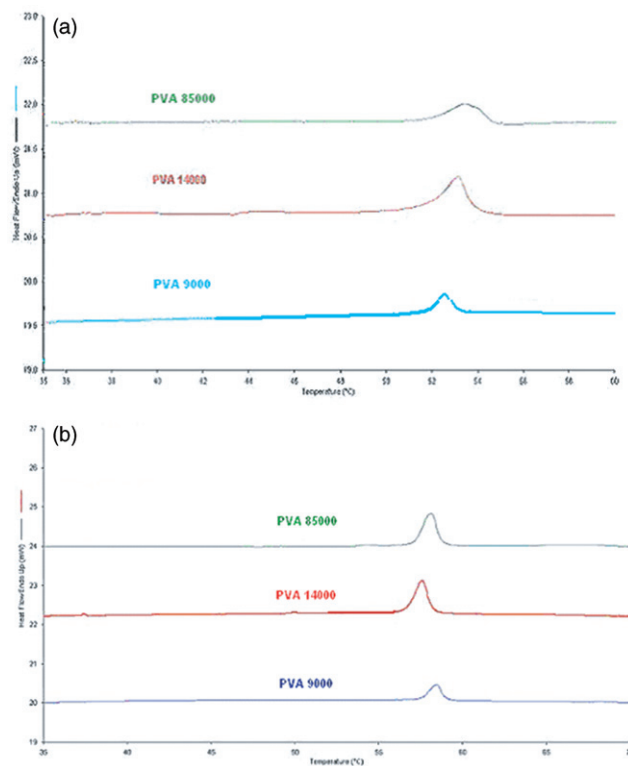
Figure 5. Thermograms of SA-SLN (a) and PA-SLN (b) stabilized with different PVA. (a) 1% SA-SLN suspensions stabilised with: PVA 9000, PVA 14 000, PVA 85 000; (b) 1% PA-SLN suspensions stabilised with: PVA 9000, PVA 14 000, PVA 85 000.
