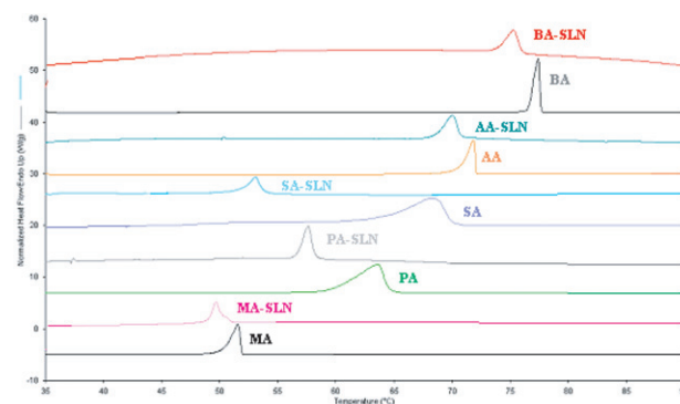
Figure 2. Thermograms of FA-SLN and bulk FA. MA: bulk myristic acid; PA: bulk palmitic acid; SA: bulk stearic acid; BA: bulk behenic acid; AA: bulk arachidic acid; MA-SLN: 1% myristic acid SLN suspension; PA-SLN: 1% palmitic acid SLN suspension; SA-SLN: 1% stearic acid SLN suspension; BA-SLN: 1% behenic acid SLN suspension; AA-SLN: 1% arachidic acid SLN suspension.
