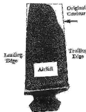
Figure 1.2: Typical damage to a compressor blade [5].
