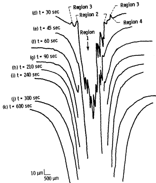
Figure 7. - Surface traces on PMMA as function of time.
