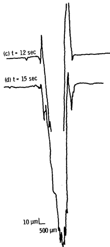
Figure 8. - Surface traces on polycarbonate as function of time.
