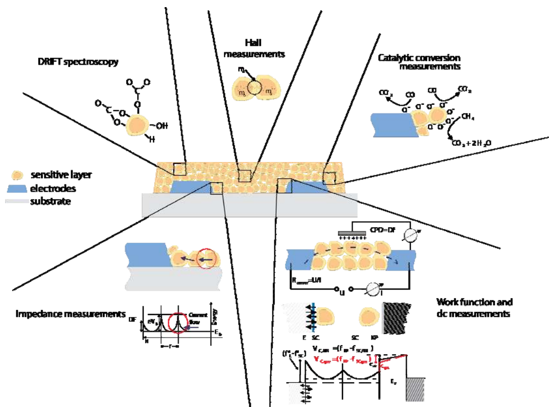
Figure 8. Operando methodology.
