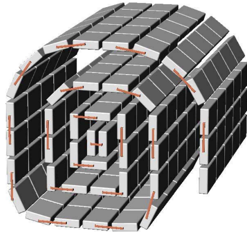
Figure 2. Low capacitance hard switch layout
