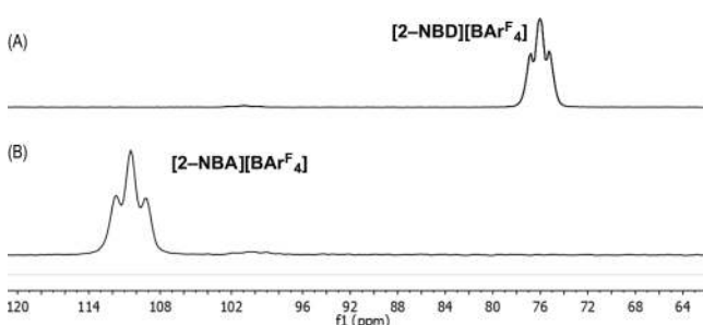
Figure 2. ^{31}\text{P}\{^1\text{H}\} SSNMR spectra of \text{H}_2 addition to powdered crystalline [2\text{-NBD}][\text{BARF}_4] . (A) [2\text{-NBD}][\text{BARF}_4] , 298 K. (B) \text{H}_2 addition (4 atm), 2 h, 298 K to form [2\text{-NBA}][\text{BARF}_4] .
