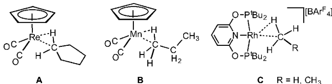
Chart 1. Representative \sigma -Alkane Complexes Characterized by Low-Temperature NMR Spectroscopy
