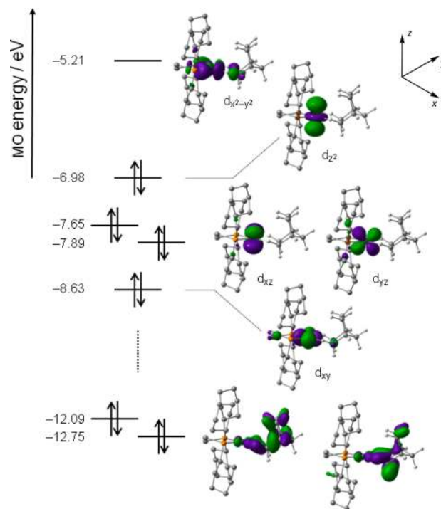
Figure 11. Key computed molecular orbitals of the [2\text{-NBA}]^+ cation. Orbital energies are in eV, and boundary surfaces are drawn with a cutoff of 0.05 \text{\AA}^{-3} .
