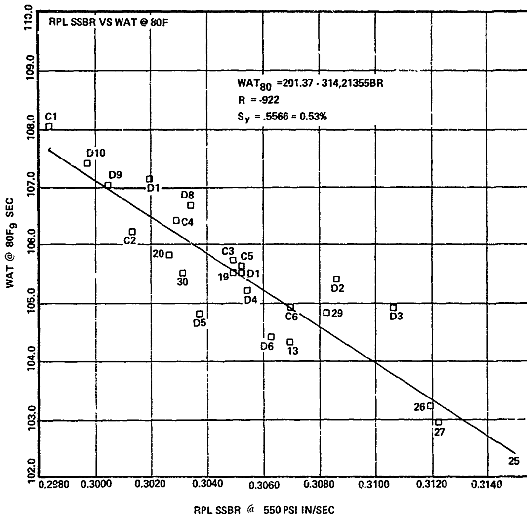
Figure 11. AFRPL Solid Strand Burn Rate (SSBR) Versus Full-Scale Motor Web Action Time (WAT)
