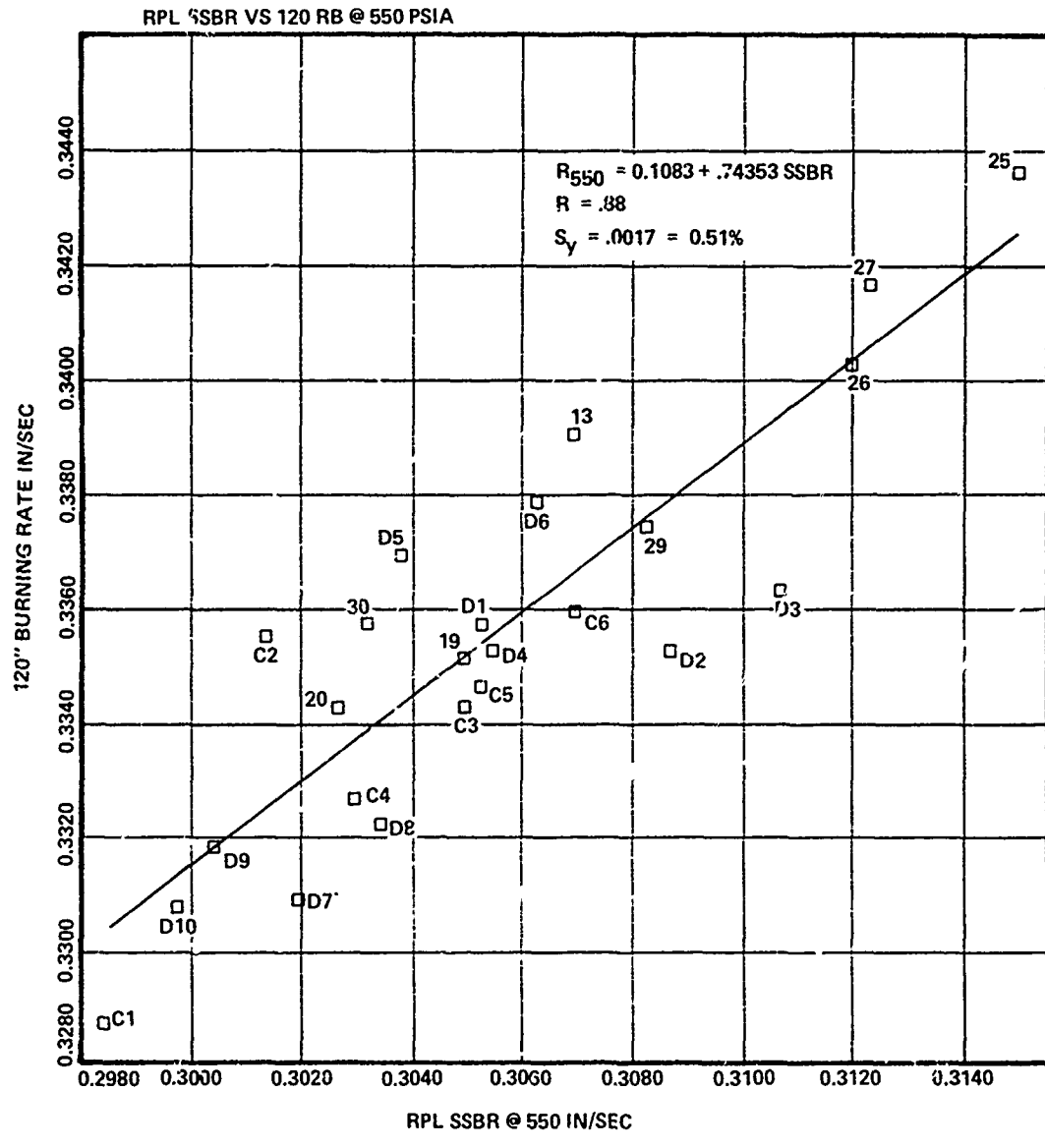
Figure 12. AFRPL Solid Strand Burn Rate Versus Full-Scale Motor Burn Rate @ 550 Psia
