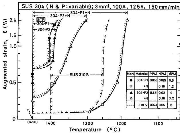
Fig. 2 Effect of N content or δ-ferrite content on ductility curves of BTR for weld metals of SUS 304 type steels containing 0.056 and 0.121%P.
