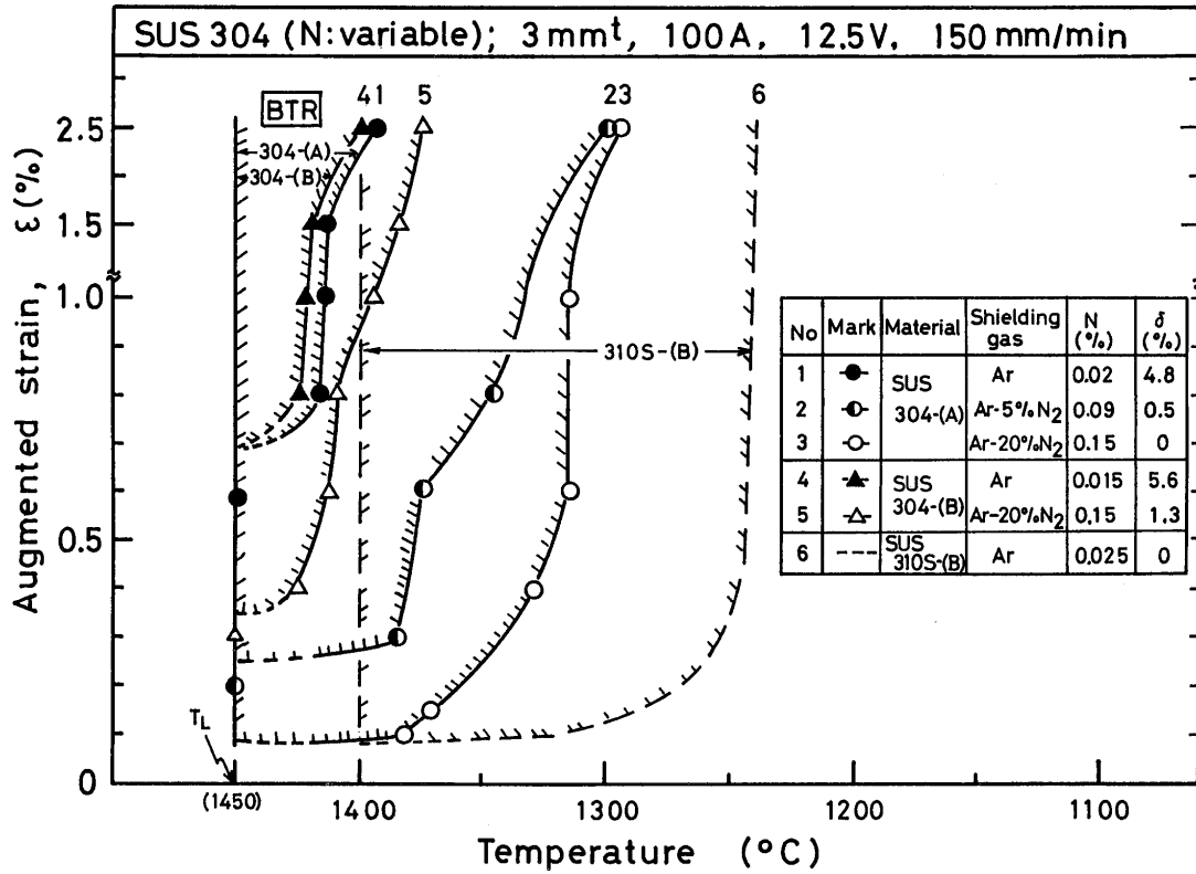
Fig. 1 Effect of N content or δ-ferrite content on ductility curves of BTR for weld metals of commercial SUS 304 steels.
