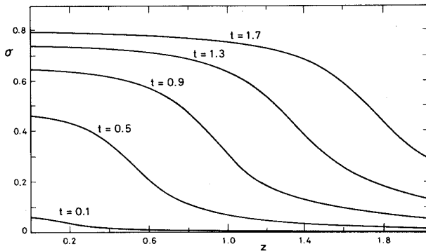
FIG. 1. This shows the function \sigma^{(-)}(z, t) for different values of t , as defined by Eq. (4.4). The origin is z = 0 and the width parameter is w = 0.2 . The function is unchanged if one reverses the sign of z . When \sigma approaches 1, the corresponding soliton solution approaches the seed metric.
