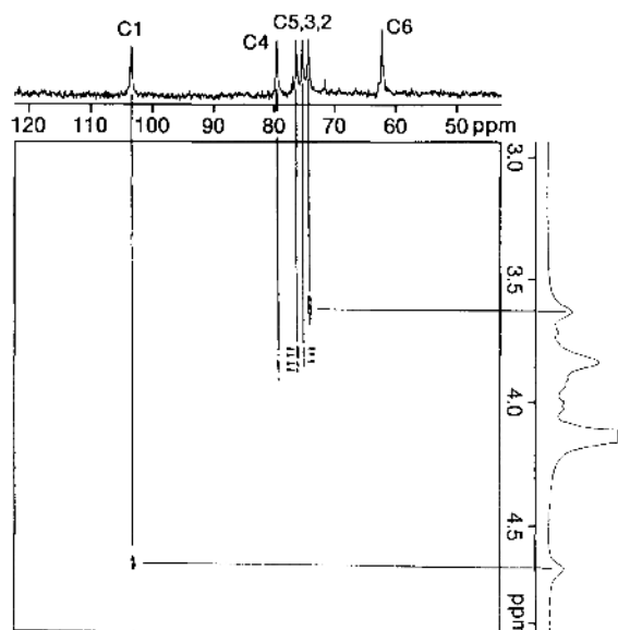
Figure 6. ^{13}\text{C} - ^1\text{H} COSY spectrum of hydrolyzed regenerated cellulose with DP_n=30 in \text{Ca}(\text{SCN})_2\text{-D}_2\text{O} at 100^\circ\text{C} . Horizontal and longitudinal axes are ^{13}\text{C} and ^1\text{H} chemical shifts and projections on the axes are ^{13}\text{C} and ^1\text{H} NMR spectra, respectively.
