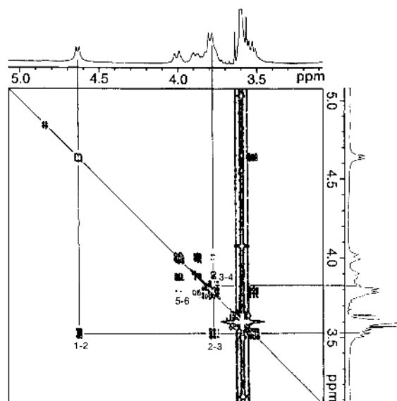
Figure 7. ^1\text{H} - ^{11}\text{C} COSY spectrum of hydrolyzed regenerated cellulose with DP_n=30 in \text{NaSCN-D}_2\text{O} system at 100^\circ\text{C} .
