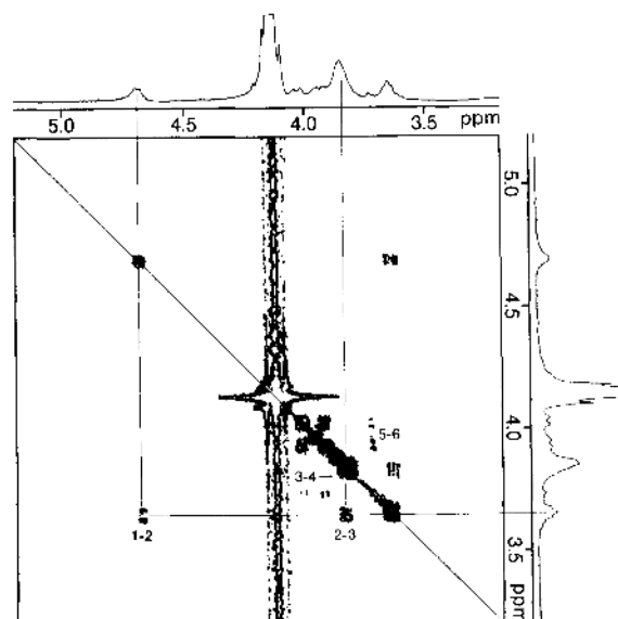
Figure 5. ^1\text{H}\text{-}^1\text{H} COSY spectrum of hydrolyzed regenerated cellulose with DP_v=30 in \text{Ca}(\text{SCN})_2\text{-D}_2\text{O} system at 100^\circ\text{C} .
