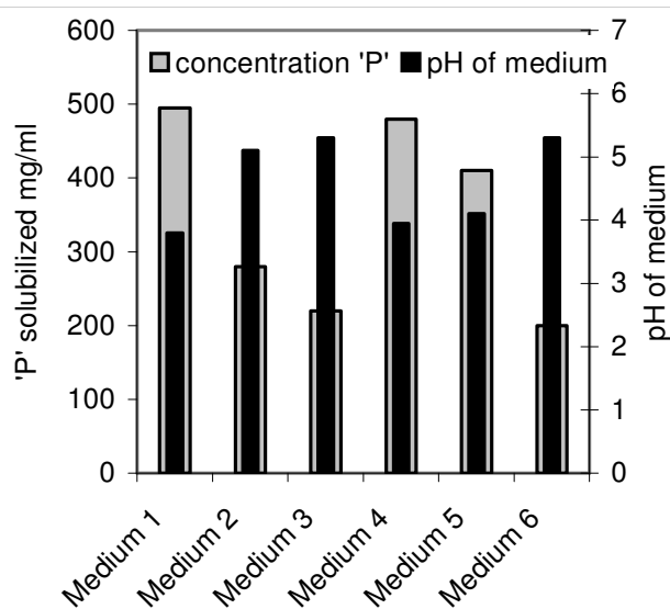
Figure 1. Effect of different media on 'P' solubilization.
