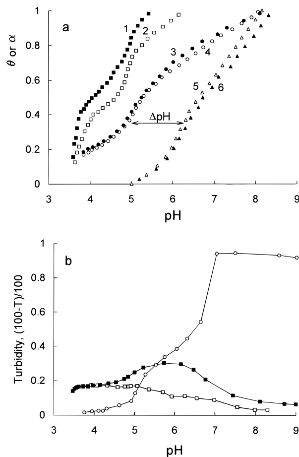
Figure 1. (a) Dependencies of the degree of conversion ( \theta ) in the polyion coupling reactions ( \blacksquare , \square , \circ , \bullet ) and degree of ionization ( \alpha ) of polyacid samples ( \triangle , \blacktriangle ) for the following systems: ( \blacksquare ) PEO-PMA - and long PEVP + ; ( \square ) PEO-PMA - and short PEVP + ; ( \circ ) PMA - and short PEVP + ; ( \bullet ) PMA - and short PEVP + in the presence of PEO; ( \triangle ) PEO-PMAA; ( \blacktriangle ) PMAA. The pH shift, \Delta\text{pH} , between the \theta -pH and \alpha -pH dependencies is shown for the PMAA complex as an example. (b) Turbidity in the systems containing complexes formed between ( \blacksquare ) PEO-PMA - and long PEVP + , ( \square ) PEO-PMA - and short PEVP + , and ( \circ ) PMA - and short PEVP + . Turbidity is determined as (100 - T)/100 , where T is transmittance (%). (a, b) The concentrations of polyions and PEO homopolymer (MW 8000) is 7 \times 10^{-4} base-moles/L.
