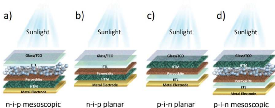
Fig. 18 (a) Mesoscopic n-i-p, (b) planar n-i-p, and (c) planar p-i-n and mesoscopic p-i-n PSC structures.
