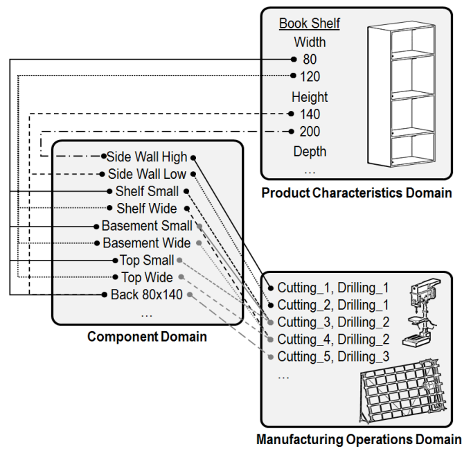
Figure 4. Combined Product and Process Configuration acc. to [24]
