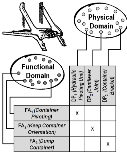
Figure 3. Mapping of functional requirements to design parameters in a design matrix
