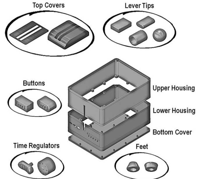
Figure 10. Modular adaptable Toaster Housing
