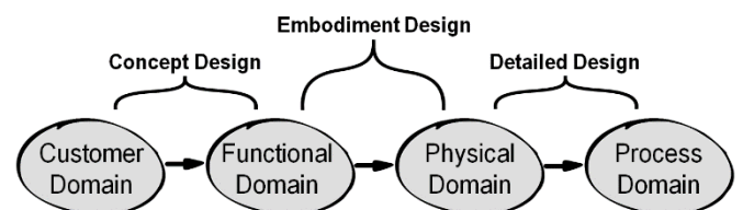
Figure 2. Domain Concept of Axiomatic Design (acc. to [21])
