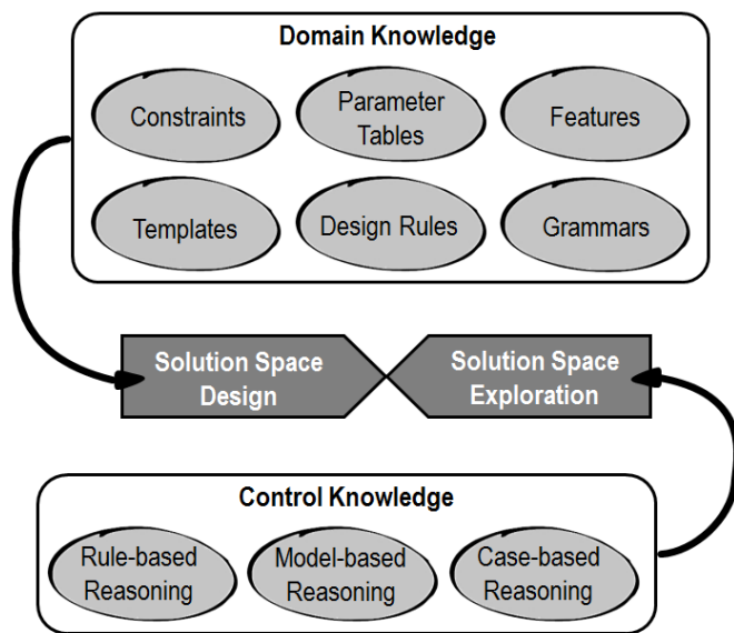
Figure 7. Knowledge Modelling in KBE and KBD
