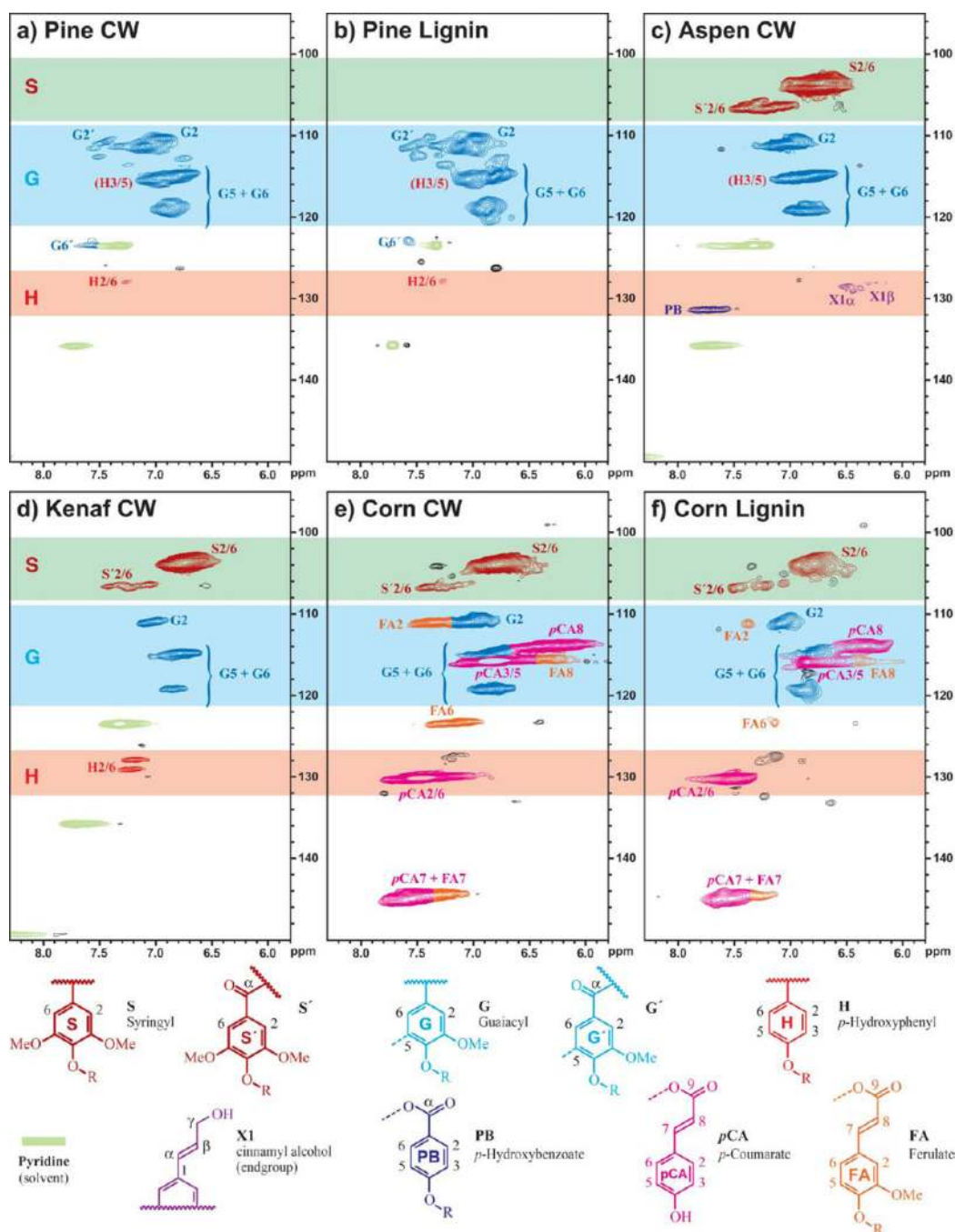
Fig. 3. Aromatic regions of 2D ^{13}\text{C} - ^1\text{H} correlation (HSQC) spectra from cell wall gels and soluble lignins from various samples in \text{DMSO-}d_6/\text{pyridine-}d_5 (4 : 1). a) Pine, b) pine isolated lignin, c) aspen, d) kenaf bast fiber, e) corn stems, f) corn isolated lignin. Correlations from the aromatic rings are well dispersed and can be categorized by the type of aromatic units (syringyl S, guaiacyl G, p -hydroxyphenyl H, p -hydroxybenzoate PB, p -coumarate p CA, and ferulate FA; color coding is according to the structures shown. Corn samples used high- d (“100%”) pyridine.
