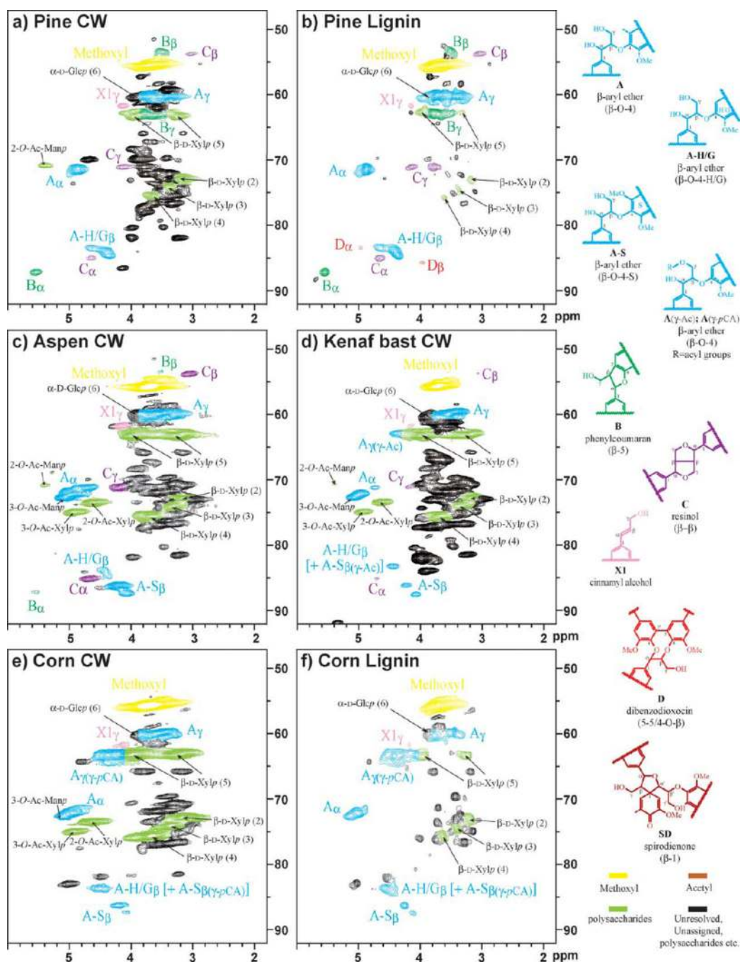
Fig. 2. Aliphatic (sidechain) regions of 2D ^{13}\text{C} - ^1\text{H} correlation (HSQC) spectra from cell wall gels and soluble lignins from various samples in \text{DMSO-}d_6/\text{pyridine-}d_5 (4 : 1). a) Pine, b) pine isolated lignin, c) aspen, d) kenaf bast fiber, e) corn stems, f) corn isolated lignin. Correlations from lignin components, and some of the characteristic polysaccharide correlations such as those from O -acetylated xylans and mannans, are well isolated from the other densely packed polysaccharides peaks; color coding is according to the structures shown.
