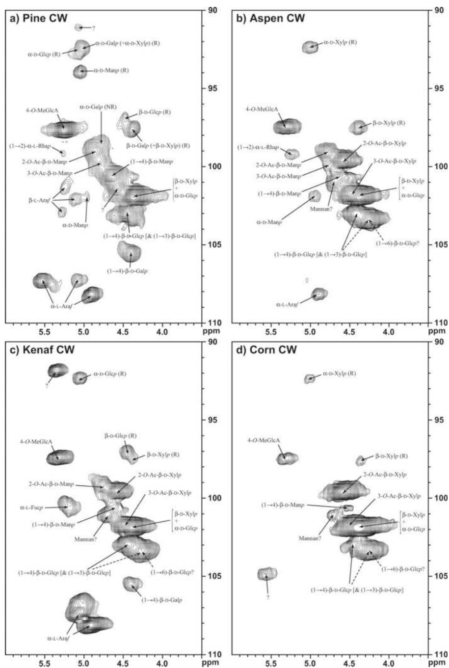
Fig. 4. Polysaccharide anomeric regions of 2D ^{13}\text{C} - ^1\text{H} correlation (HSQC) spectra from cell wall gels from various samples in \text{DMSO-}d_6/\text{pyridine-}d_5 (4 : 1). a) Pine, b) aspen, c) kenaf bast fiber, d) corn stems. The tentative assignments are based on actual NMR data from limited sources of polysaccharides in \text{DMSO-}d_6/\text{pyridine-}d_5 (4 : 1) and other references in which samples were mostly in \text{D}_2\text{O} . \alpha -D-Glcp, \alpha -D-glucopyranoside; \beta -D-Glcp, \beta -D-glucopyranoside; \alpha -D-Manp, \alpha -D-mannopyranoside; \beta -D-Manp, \beta -D-mannopyranoside; \beta -D-Xylp, \beta -D-xylopyranoside; \alpha -D-Galp, \alpha -D-galactopyranoside; \beta -D-Galp, \beta -D-galactopyranoside; \alpha -L-
