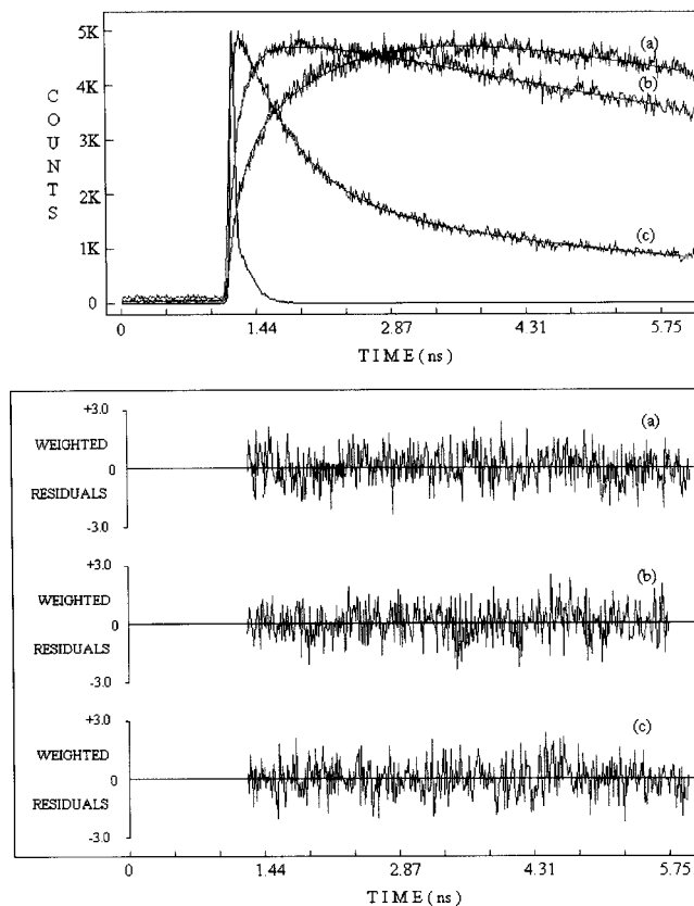
Figure 2. Fluorescence decays of 4-AP in 0.27 M TX in benzene/ n -hexane (3:7, v/v), R = 5 , at (a) 600 nm, (b) 510 nm, and (c) 450 nm.
