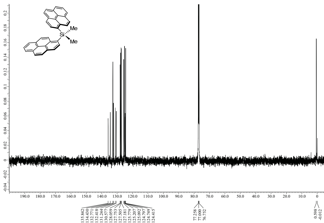
Fig. S4. 126 MHz ^{13}\text{C} NMR spectrum of dimethyldi(1-pyrenyl)silane in \text{CDCl}_3 .
