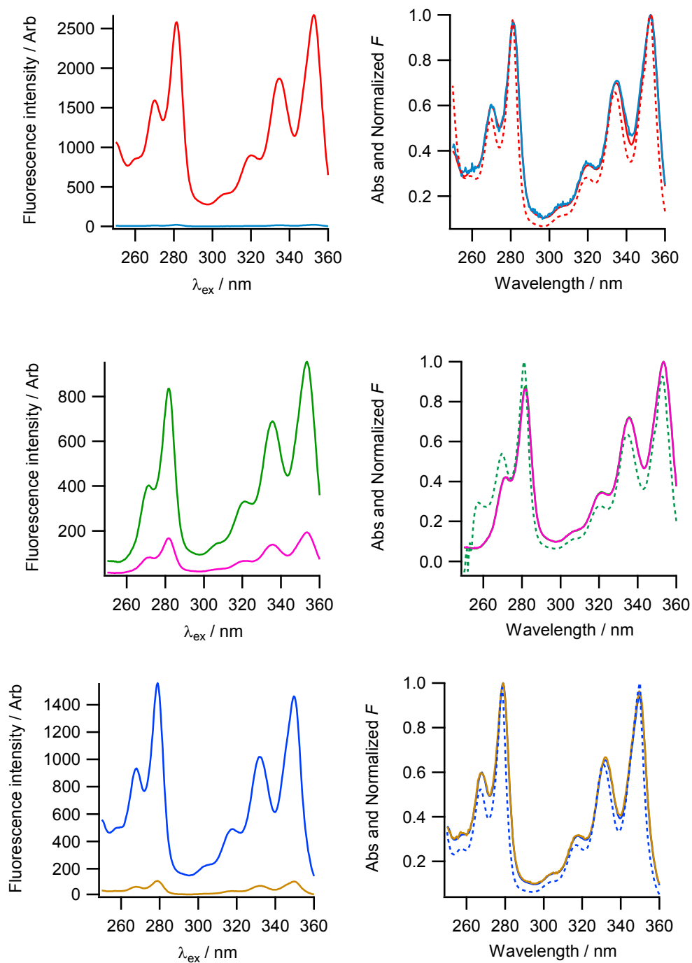
Fig. S21. (Left) Excitation spectra of 1c in \text{CHCl}_3 at 379 (—) and 470 nm (—), in DMSO at 379 (—) and 470 nm (—), and in MeCN at 379 (—) and 470 nm (—), respectively. (Right) UV-vis spectra of 1c in the corresponding solvents were overlapped as dotted lines to the normalized fluorescence spectra, respectively.
