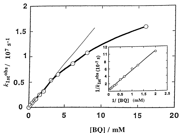
Fig. 6. First-order decay rate constants ( k_{1st}^{\text{obs}} ) of {}^3(\text{RB}^{2-})^* in 1-butanol as a function of [BQ]. Inset: 1/k_{1st}^{\text{obs}} vs. 1/[\text{BQ}] .
