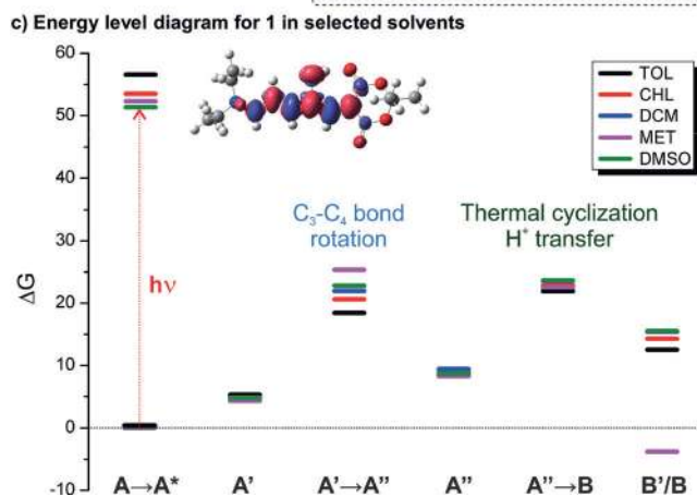
Figure 1. Donor-acceptor Stenhouse adducts: a) photoswitches used herein; b) proposed photoswitching mechanism [15,16] and c) corresponding energy level diagram in kcal mol -1 for 1 in selected solvents obtained at the M06-2X/6-31+G(d)/SMD level of theory. Analogous diagrams for 2 and 3 are presented in the SI (Figure S8.5). In the electronic density difference (EDD) plot (inset), the blue (red) regions correspond to a decrease (increase) in electron density upon electronic excitation. The energy levels of the product correspond to B and B' structures in aprotic and protic solvents, respectively.
