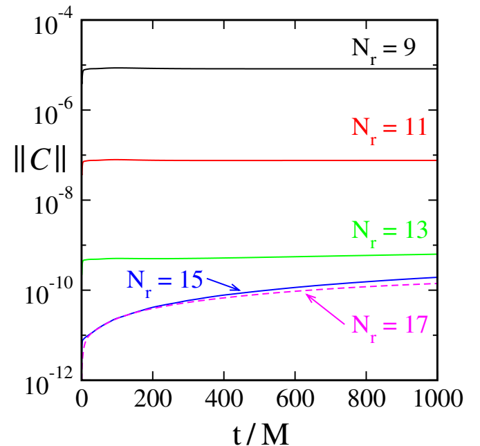
FIG. 5 (color online). Constraint violations in dual-coordinate-frame evolutions of Schwarzschild, with comoving coordinates that rotate uniformly with angular velocity \Omega = 0.2/M . These evolutions use the new rotating-frame tensor-spherical-harmonic filtering algorithm. The highest resolution case (dashed curve) uses more angular basis functions ( \ell \leq 13 instead of \ell \leq 11 ) as a more stringent test of convergence.
