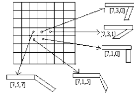
Figure 6. Some of the landmarks coded by the Kohonen neurons. The weight vector is shown along with landmarks.
