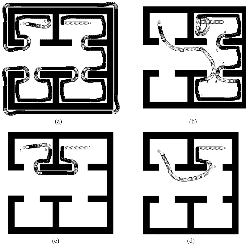
Figure 16. (a) According to the earlier method the robot switches from 'T' to H mode at point 'b' when points a, b and c are almost collinear. (b) A more reduced path results by the current method. (c) The robot tracks the obstacle in counter clockwise direction. (d) Path obtained when the earlier algorithm modified with the new criteria for switching from T mode to H mode.
