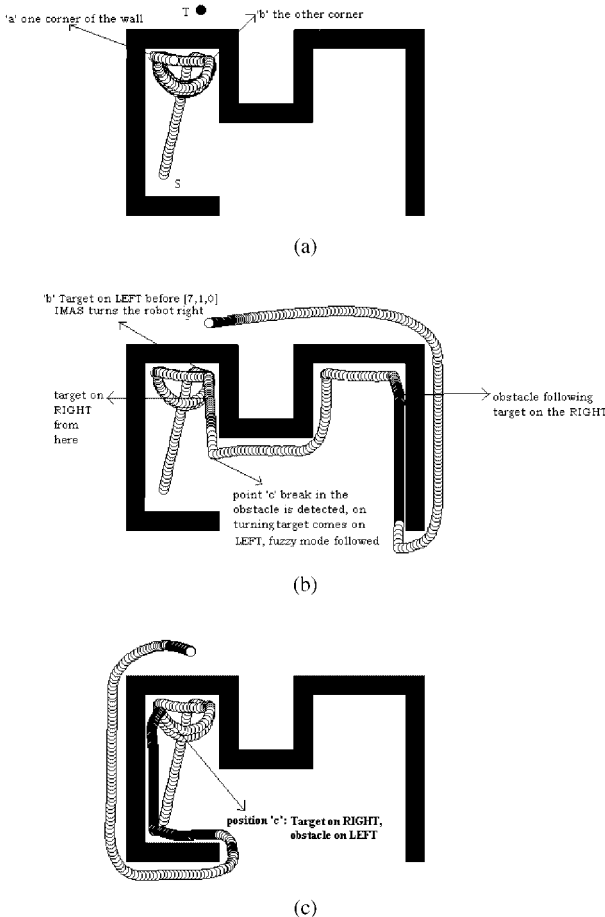
Figure 10. (a) The robot getting trapped between the two corners 'a' and 'b' though IMAS acts making the robot turn appropriately at 'b'. (b) Robot guided out by DMAS. (c) Fuzzy ART detects local minima ([7,8,5]) earlier than SOM, invokes DMAS. A shorter path results.
