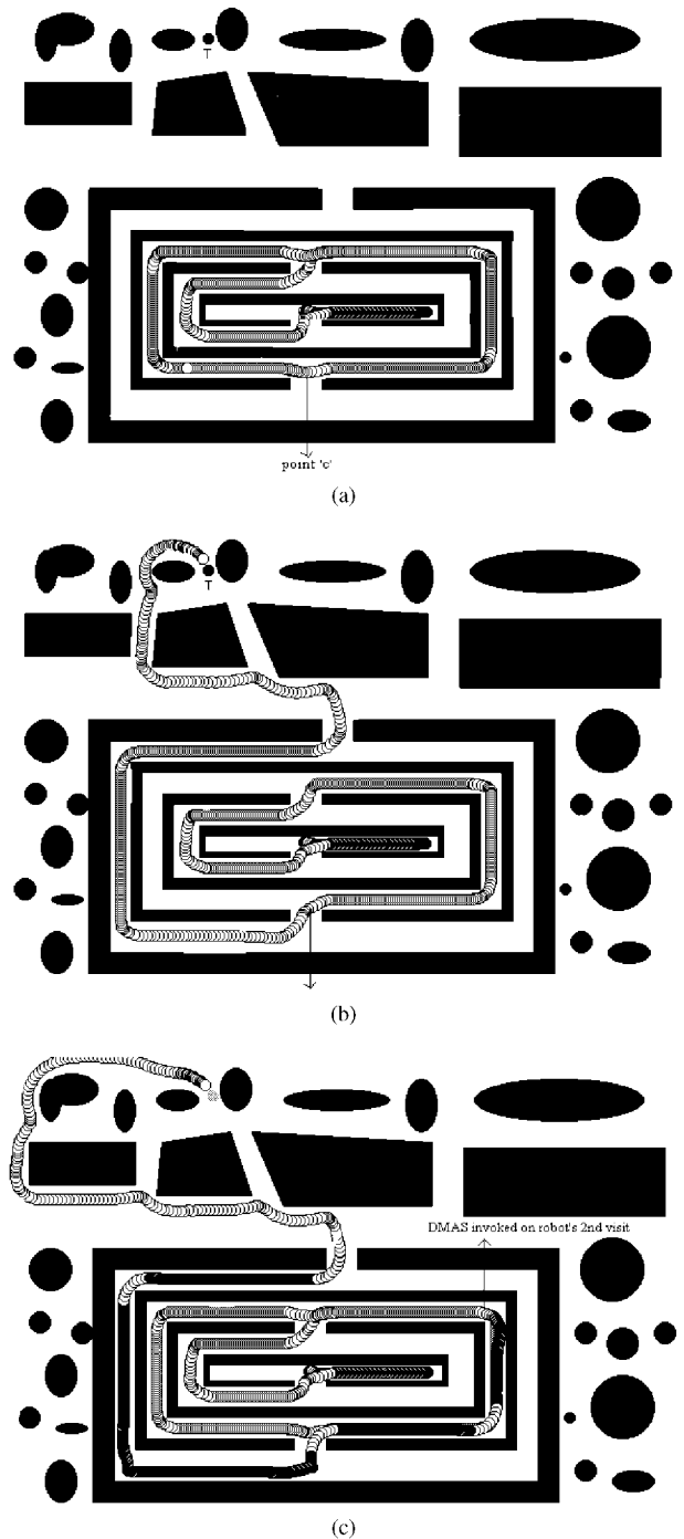
Figure 13. (a) Point 'c' robot unable to pull itself out because of conflicting target attracting and obstacle avoidance behaviors. (b) IMAS for [3, 4, 8] pulls the robot out of the maze. Absence of IMAS is seen as robot completes a full traversal between the 2nd and 3rd obstacle loops from the center. (c) Without SOM, Fuzzy ART pulls the robot out of the maze. Absence of IMAS is seen as robot completes a full traversal between the 2nd and 3rd obstacle loops from the center.
