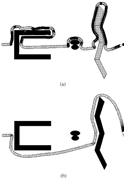
Figure 15. (a) An example from a previous paper. Heuristic determination results in misidentification of a situation to a local minima. (b) The robot traverses a shorter path by the current method.
