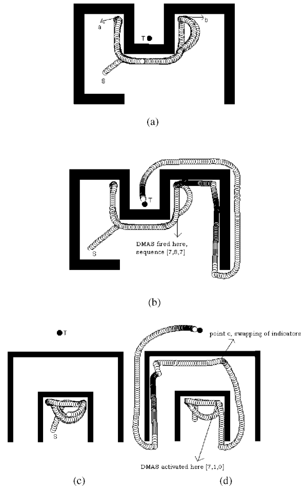
Figure 11. (a) Another infinite loop. Robot oscillating between ‘a’ and ‘b’. (b) Robot guided out of oscillations. (c) Double walled obstacle. (d) Guiding out of the double layered wall.
