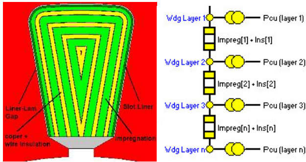
Fig. 3: Layered winding model suitable for electric machines
