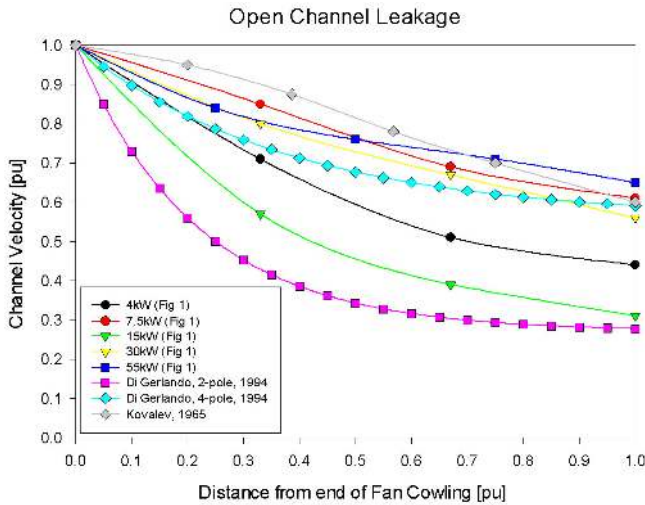
Fig. 7: Typical form reduction in local fin channel air velocity with distance from the fan
