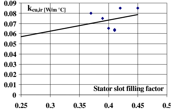
Fig.2: Equivalent thermal conductivity in the stator slots.
