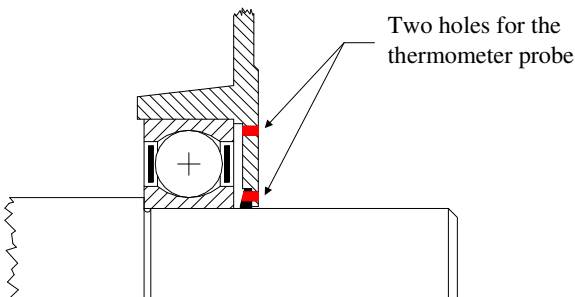
Fig.11: Adopted system for the bearing temperature measurement.
