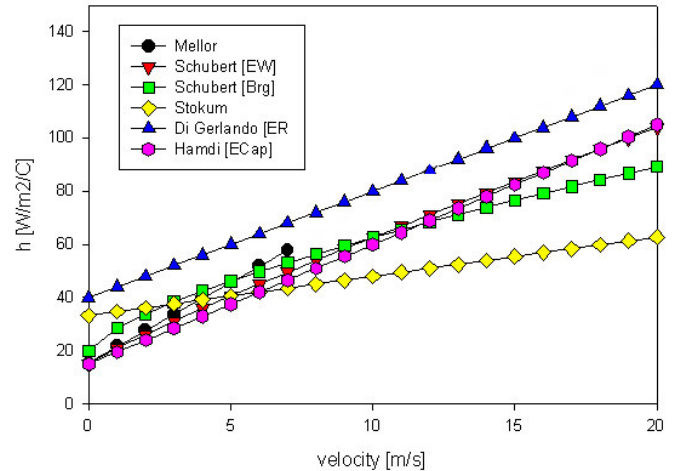
Fig 9: Published End Space Convection Correlations
