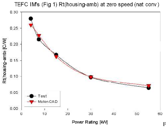
Fig. 4: Natural convection resistance between frame and ambient air
