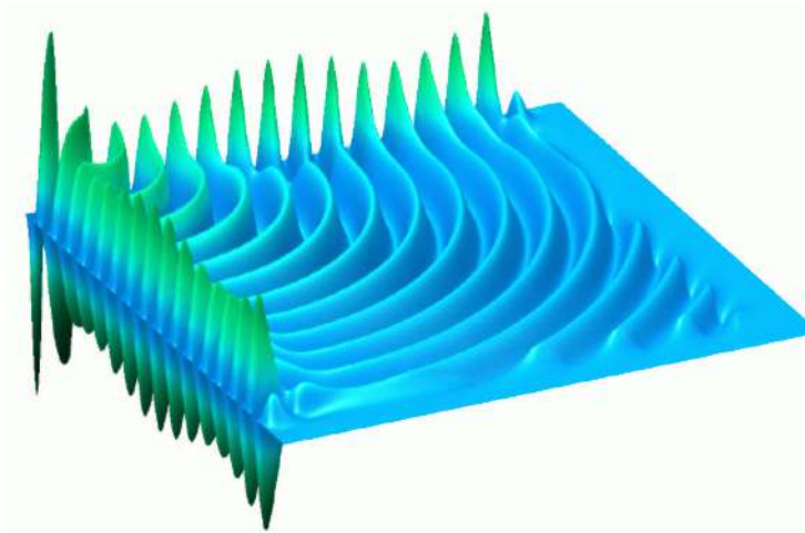
Figure 5. Real part of a representative radial function for electron-hydrogen scattering at 17.6 eV incident energy. Vertical axis is Re(\Psi) and the two horizontal axes are r_1 and r_2 with origins at the rear left corner. \Psi_{l_1, l_2}^L(r_1, r_2) is shown for singlet spin, L = 2 and l_1 = l_2 = 1
