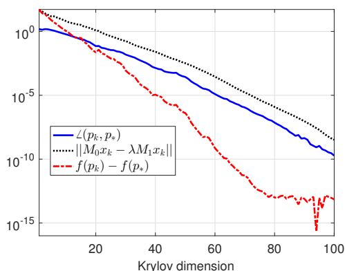
FIG. 6. Accuracy in solution \angle(p_k, p_*) and objective value f(p_k) - f(p_*) as Krylov subspace dimension k varies. Also shown is the residual \|M_0x - \lambda M_1x\|_2 of the approximate eigenpair.
