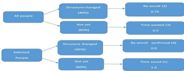
Figure 6. Decision tree of structural change due to cataract.
