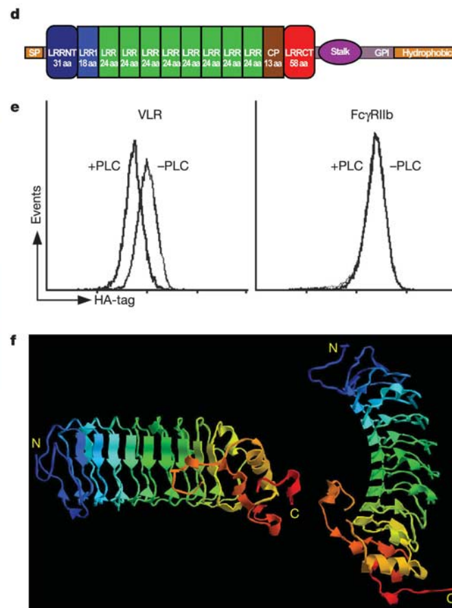
kilobases. d , VLR stick model. Sections from left to right are: signal peptide, N-terminal LRR, nine LRRs, connecting peptide, C-terminal LRR, threonine/proline-rich stalk, GPI anchor and hydrophobic tail (clone 12.26, AY577974). e , Epitope-tagged VLR and Fc \gamma RIIb (control) expressed in mouse thymoma cells, treated with (+PLC) or without (-PLC) GPI-phospholipase C. f , Three-dimensional model of VLR diversity region (two rotations).
