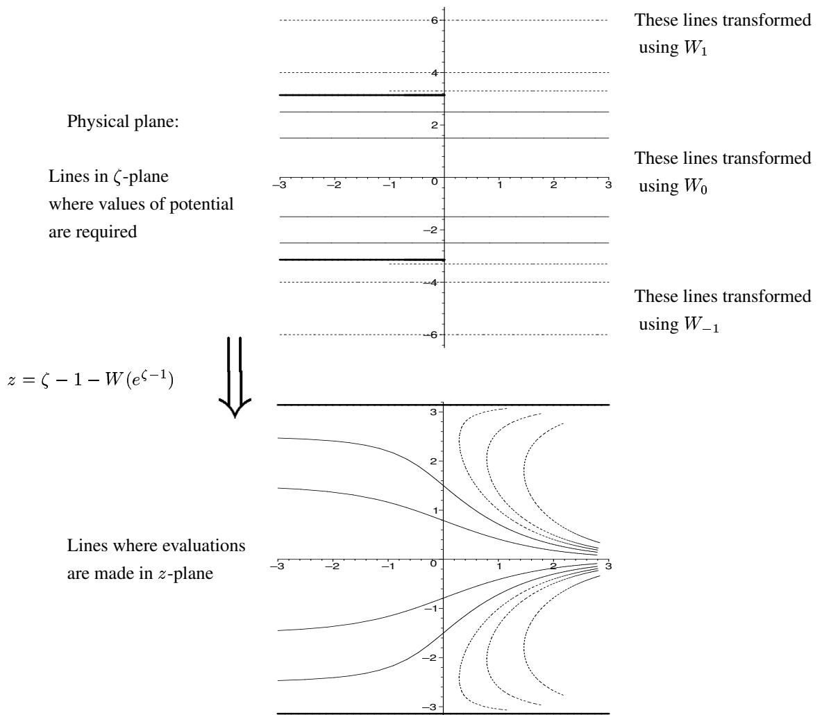
Fig. 2. The top and bottom sets of axes again show the \zeta - and z -planes. Now the transformation proceeds from top to bottom using the inverse mapping z = \zeta - 1 - W_{\kappa(\zeta)}(e^{\zeta-1}) .
