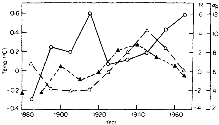
Figure 1. Decadal anomalies of monsoon season rainfall, its standard deviation and the decadal anomalies of northern hemisphere surface temperature.
