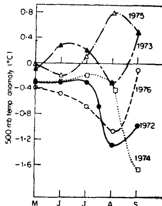
Figure 5. Year-to-year variations in the 500 mb temperature anomaly averaged for the longitudinal belt 30–120° E along 30° N.
