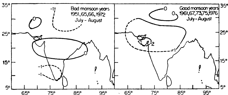
Figure 2. Sea-level pressure anomaly (mb) patterns for the composites of bad and good monsoon rainfall years over India.
