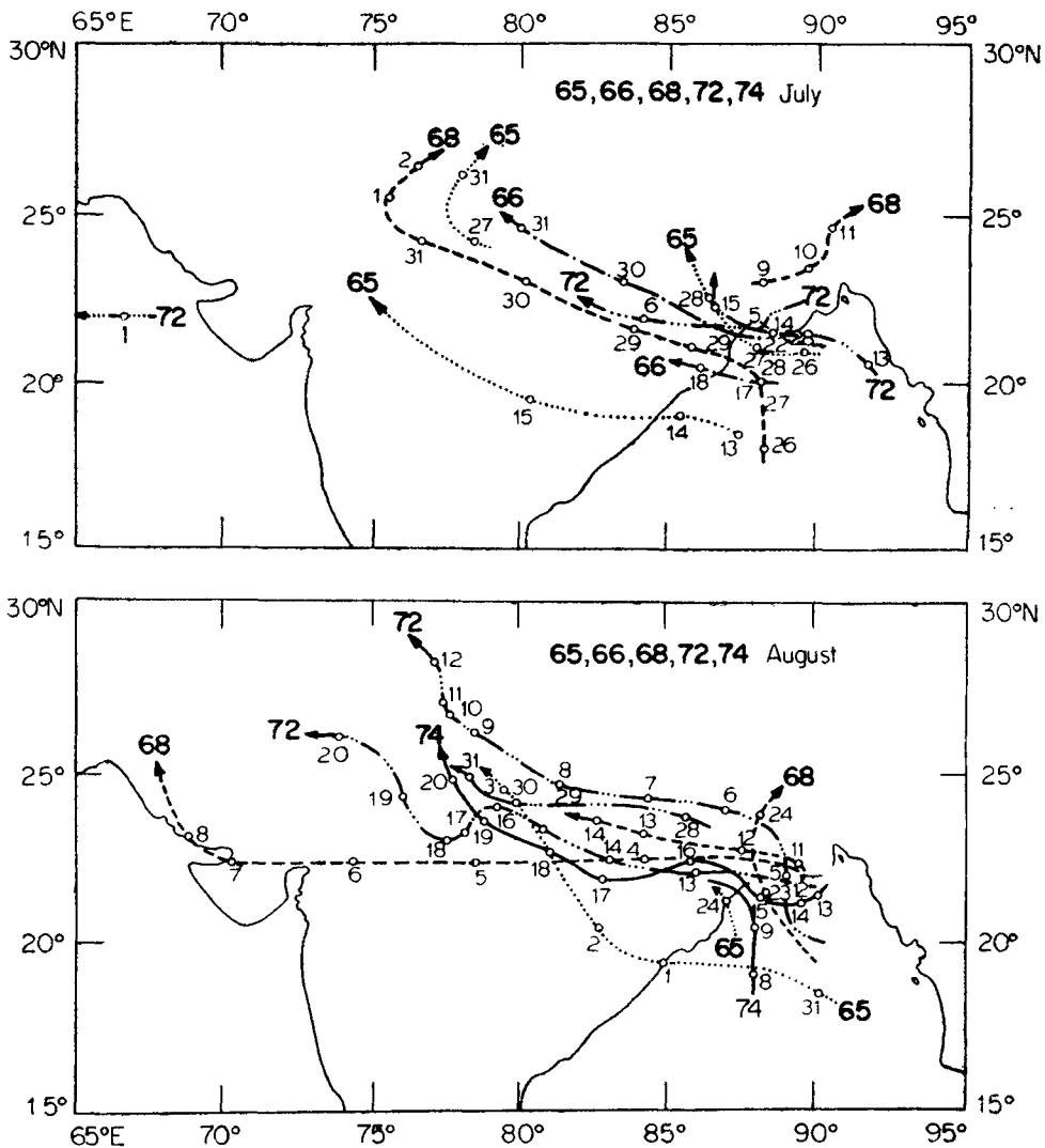
Figure 4a. Tracks of monsoon depressions for the months of July and August during bad monsoon rainfall years.
