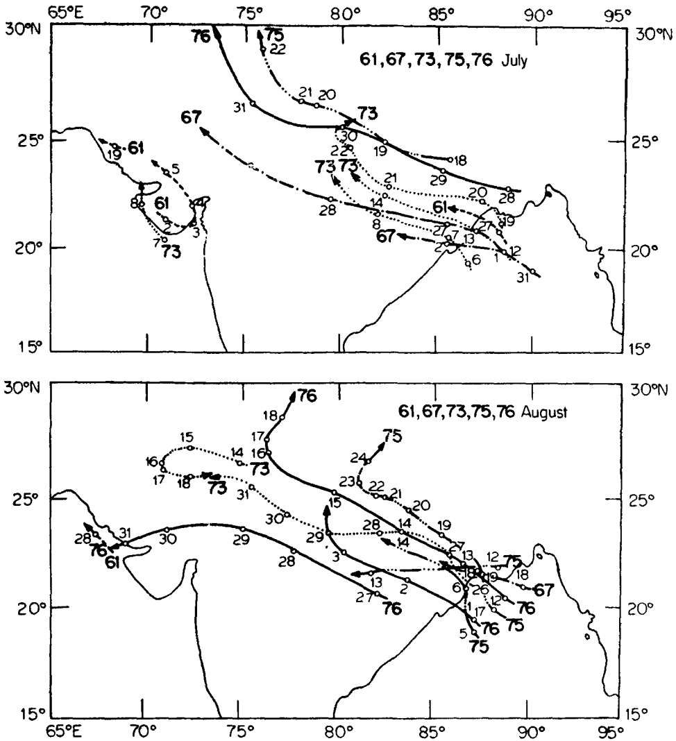
Figure 4b. Tracks of monsoon depressions for the months of July and August for the good monsoon rainfall years.
