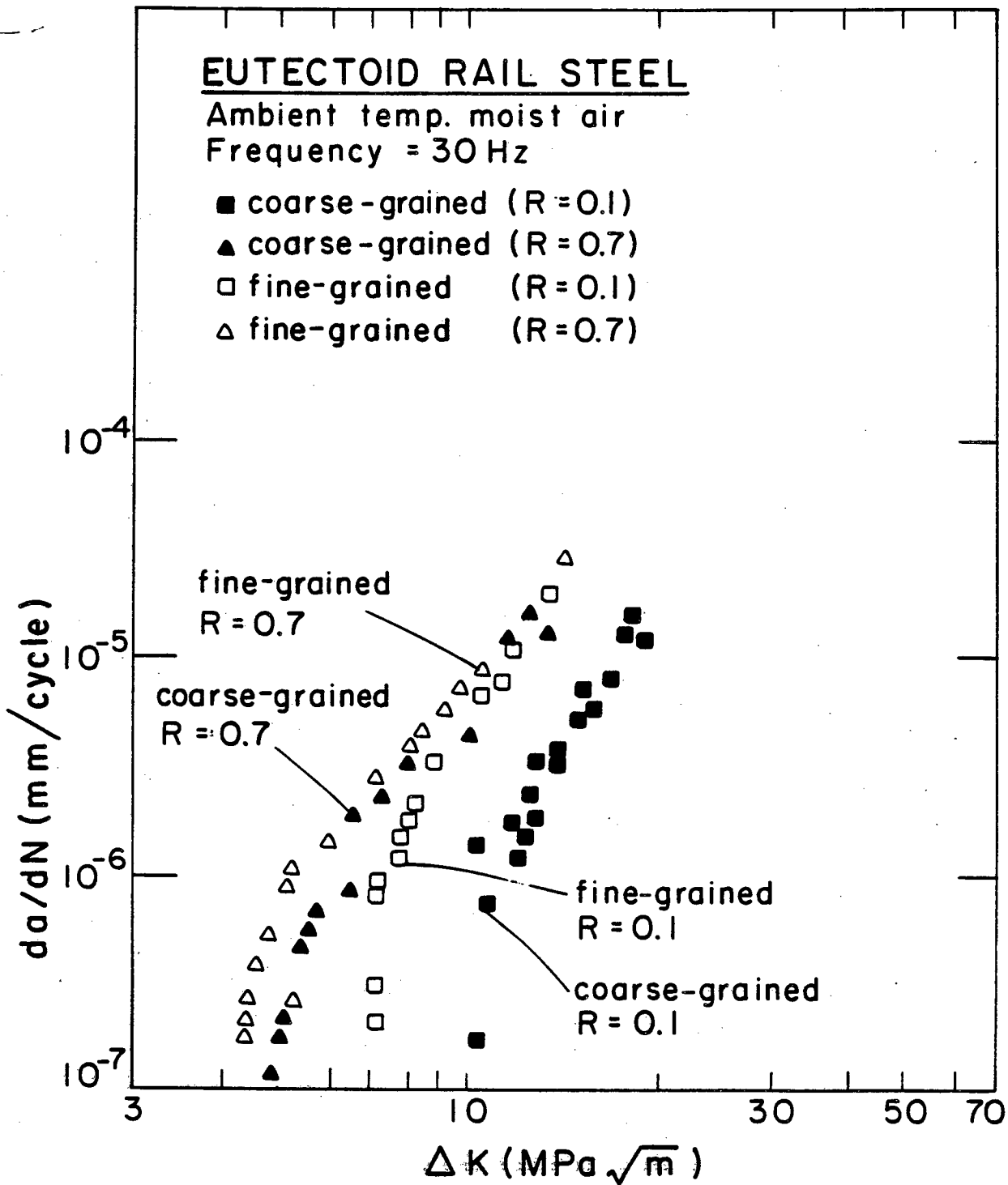
Fig. 5. Fatigue crack propagation in fully pearlitic hot-rolled rail steel ( R = 0.1 and 0.7 ), showing lower growth rates and higher threshold values in the coarse-grained microstructure ( d = 130\mu m ) compared to the fine-grained structure ( d = 25\mu m ), at low load ratios only (after ref. 11).
