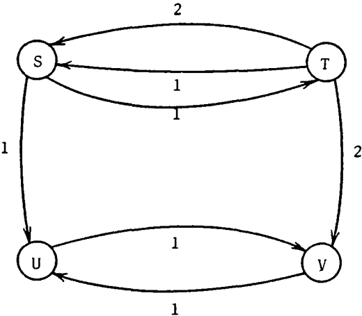
Fig. 1 Example of a system in which process P2 can deadlock. The set of states is \Sigma = \{S, T, U, V\} , and the set of processes is \Pi = \{P1, P2\} .
