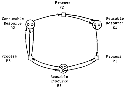
FIG 4 Example of a state in a general resource system. R1 and R3 are reusable resources whose total units are t1 = 2 and t3 = 3 R2 is a consumable resource whose only producer is P2 . The available units are r1 = 1 , r2 = 2 , and r3 = 0 . The state is not deadlocked because it can be reduced by P1 , then by P2 , and then by P3 .
