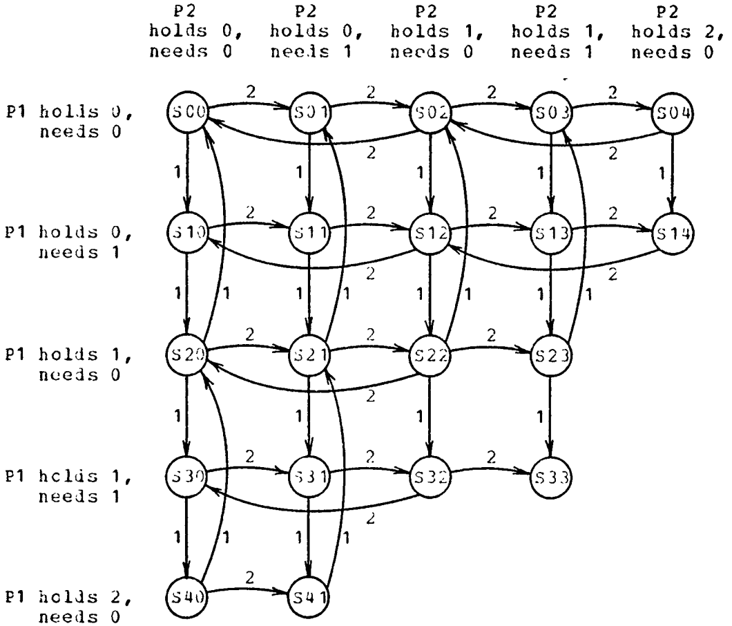
FIG 2 A system with two processes and a resource of two identical units.
