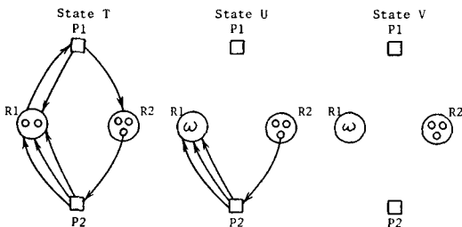
FIG 6 Reductions of a general resource graph. (State T is identical to state T in Figure 5) R1 is a consumable resource, and R2 is a reusable resource. State T is reduced by P1 to obtain U , and U is reduced by P2 to obtain V . T is completely reducible because the reductions delete all edges, therefore, T is not a deadlock state
