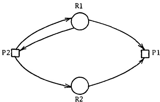
FIG 7. Example of a claim limited graph for a claim limited consumable resource system
