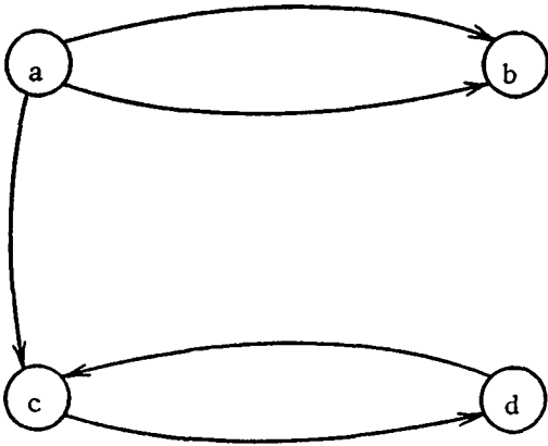
FIG 3. An example of a bipartite directed graph.
