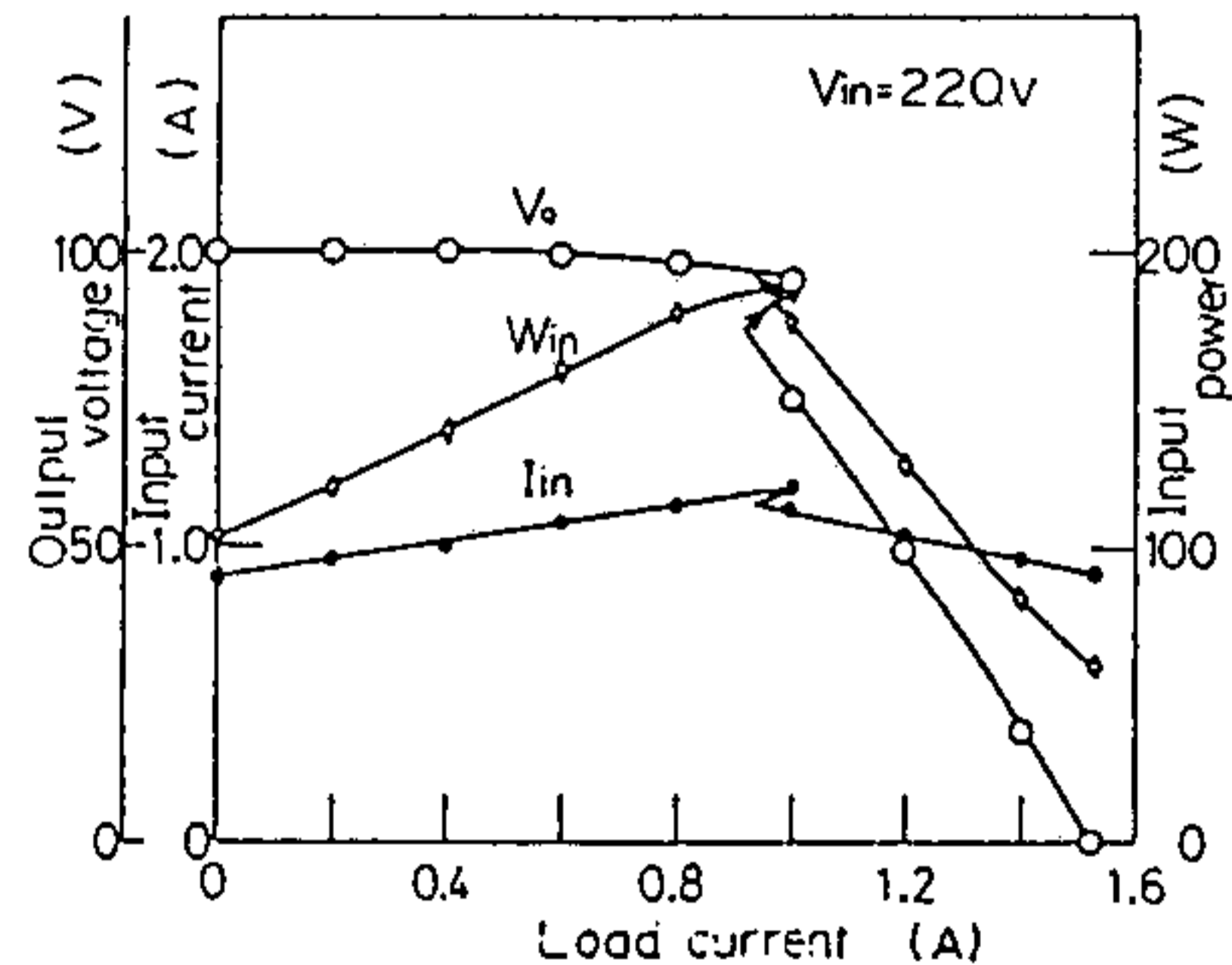
Fig.7 Load characteristics
