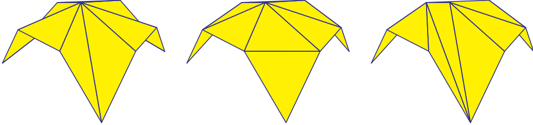
FIGURE 10. Three control polytopes.
