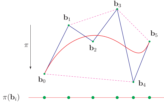
FIGURE 5. A compatible projection.
