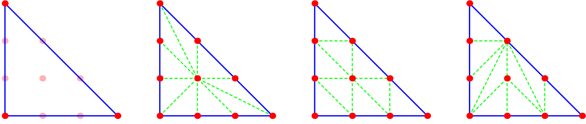
FIGURE 8. Some regular triangulations.
