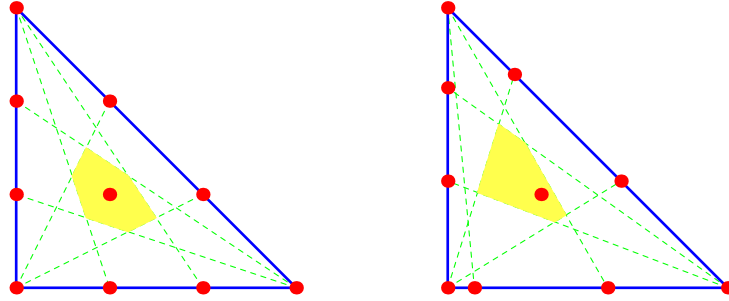
FIGURE 4. Compatible control points for the Bézier triangle.
