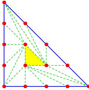
FIGURE 9. An irregular triangulation.
