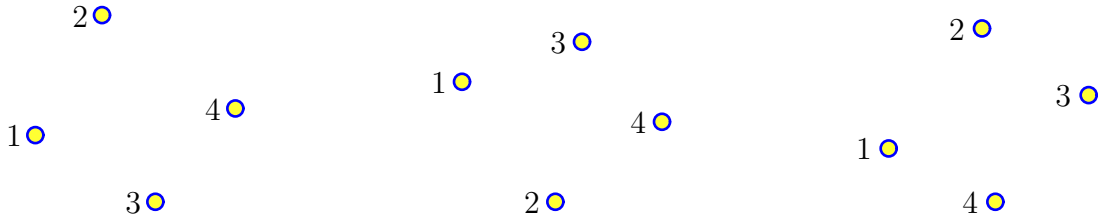
FIGURE 3. Compatible and incompatible sets of points.
