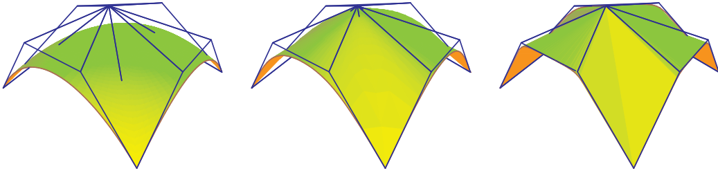
FIGURE 11. Degeneration to the control polytope.
