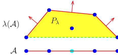
FIGURE 7. Upper faces and a regular subdivision.
