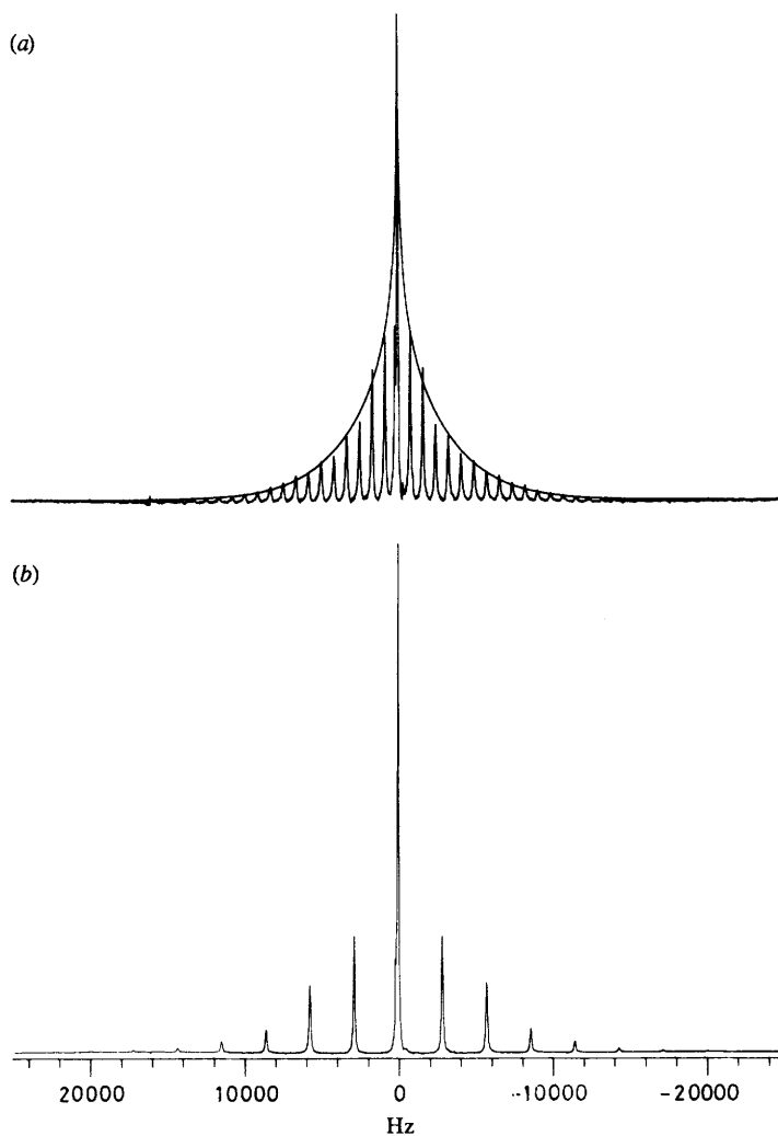
Fig. 1. 50.6 MHz ^1\text{H} Fourier-transform MAS NMR spectra of decanol (38.9%)–sodium decanoate (30.1%)– \text{D}_2\text{O} (31.0%) at 21 °C. (a) 0.82 kHz spinning speed. (b) 2.86 kHz spinning speed. Recycle times of 5 s, 32 acquisitions and 10 Hz exponential line-broadening were utilized in both spectra. Superimposed on the 0.82 kHz MAS NMR spectrum is the 'super-Lorentzian' lineshape calculated using eqn (4) with an assumed Gaussian lineshape function, f(x) = \exp(-\pi x^2) .
