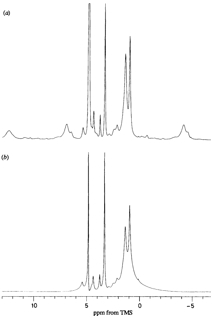
Fig. 6. 500 MHz ^1\text{H} Fourier-transform NMR spectra of egg-yolk lecithin-CHOL (1:1) at ca. 21 °C. (a) MAS NMR spectrum of a 50 wt % hand dispersion of EYL-CHOL (1:1) in ^2\text{H}_2\text{O} . (b) Conventional FT NMR spectrum of a 10 wt % sonicated dispersion of EYL-CHOL (1:1) in ^2\text{H}_2\text{O} . Recycle times of 5 s were used in both cases, as was an exponential line-broadening of 8 Hz. Note the presence of spinning sidebands in the MAS NMR spectrum and a broad, non-Lorentzian lineshape in the sonicated dispersion.
