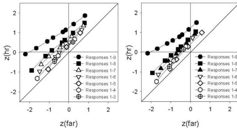
Figure 8. Item recognition zROCs cumulated across different combinations of item confidence ratings in Experiment 2. The zROCs for words are shown on the left; for travel scenes, on the right. Filled symbols: zROC curves for items with above-zero source discrimination. Unfilled symbols: zROCs for responses that carried no source information. hr = hit rate; far = false alarm rate.
