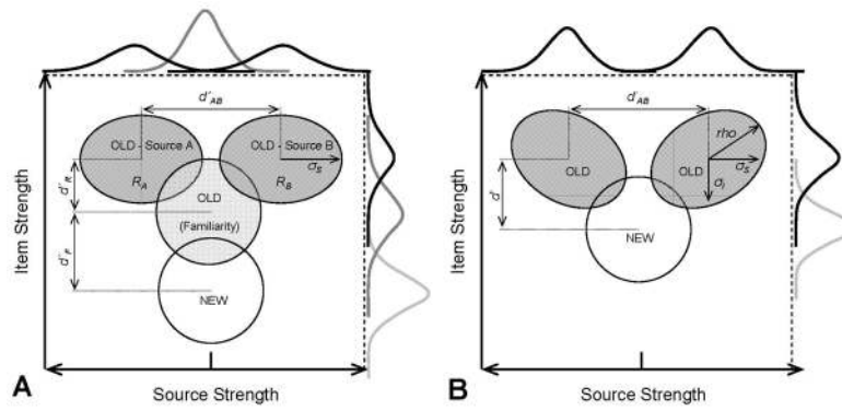
Figure 4. Two dimensional signal detection models for item and source judgments. A. The variable recollection dual process signal detection model (VRDP) leads to a natural model of conjoint item-source accuracy. The horizontal dimension reflects source strength; the vertical axis reflects item strength. Closed figures represent multivariate test probe distributions viewed from above, as in a topographic map. Recollected old probes (dark shading) lead to high item strength and also source discriminability. Old items that are not recollected do not result in source discriminability but do lead to item discriminability (light shading). New items are shown by the unshaded curve. B. The two-dimensional signal detection model proposed by DeCarlo (2003). The fact that item and source discriminability are correlated with one another requires that for very low values of item confidence, old items should show negative source discriminability as the two distributions cross.
