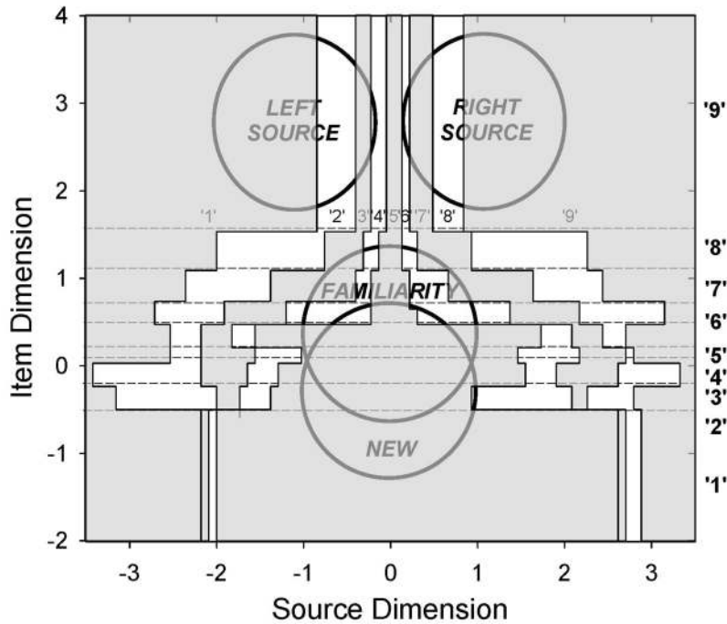
Figure 6. Graphical representation of the best-fitting parameters from the conjoint item-source ratings in Experiment 2. Item criteria are shown as horizontal lines that extend across the entire figure.
