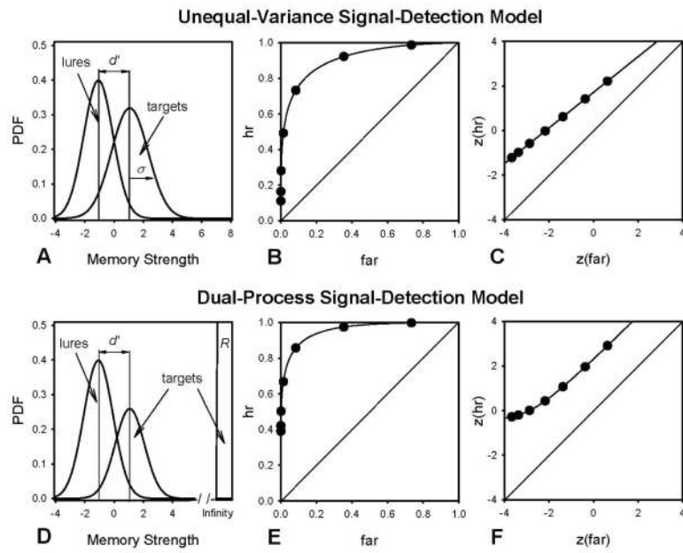
Figure 1. Probability density functions (PDF) and receiver operating characteristics (ROC) and z-transformed ROC (zROC) curves generated from the unequal-variance signal detection model (UVSD, top) and the dual-process signal detection model (DPSD, bottom). A, D. Model PDFs. B, E. ROC curve generated by the models. C, F. zROCs.
