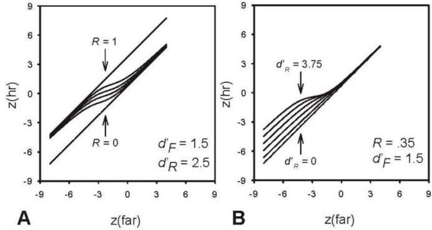
Figure 3. The effect of R and d'_R on zROC curves generated by the VRDP model. A. R was increased from 0 to 1 in increments of 0.2 (setting d'_F = 1.5 and d'_R = 2.5 ). For R = 0 and R = 1 , the z-ROC curve is a straight line with a slope of unity. For intermediate values of R , the z-ROC curve shifts from the straight line corresponding to the familiarity distribution to the straight line corresponding to the recollective distribution, with the value of R controlling the location and the steepness of the transition. B. d'_R was increased from zero to 3.75 in increments of 0.75 (fixing R = 0.35 and d'_F = 1.5 ). The value of d'_R controls the intercept of the bottom straight line.
