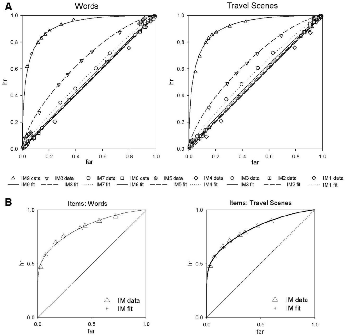
Figure 7. The VRDP model fit to conjoint item and source ROCs. A. Source memory ROCs conditional on item recognition. The open symbols are the data. The curves depict the model fit. Data from the word condition of Experiment 2 is on the left. Data from the travel scene condition is on the right. B. Fits to the item recognition ROC from the conjoint item-source fit in panel A. hr = hit rate; far = false alarm rate.
