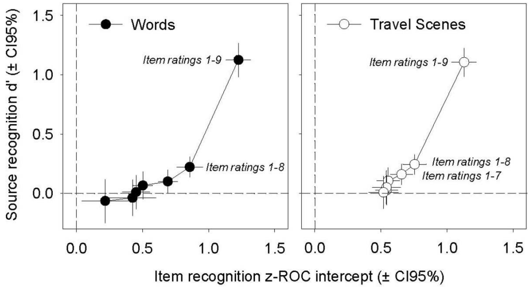
Figure 9. Source discrimination as a function of item recognition accuracy for words (left) and travel scenes (right) in Experiment 2. On the x-axis, an estimate of item discrimination (defined as the intercept of the zROC) is plotted across the cumulated item ratings along with the 95% confidence intervals. On the y-axis, source accuracy, expressed as d' is given. The rightmost point in each panel reflects item and source accuracy for all responses (i.e., item recognition confidence ratings 1 through 9). The second point from the right corresponds to estimates of item and source accuracy calculated only for probes assigned item ratings 1 through 8, and so on, with the leftmost point in each panel corresponding to probes assigned ratings 1 through 3.
