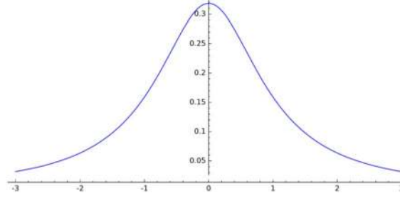
Fig. 2. The free symmetric 1-stable density (BS).
