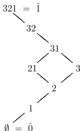
FIGURE 2. The Bruhat order for OG(3) .
