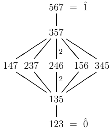
FIGURE 1. The multiplicity poset
