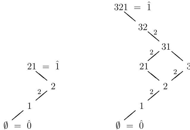
FIGURE 3. The multiplicity posets LG(2) and LG(3)
