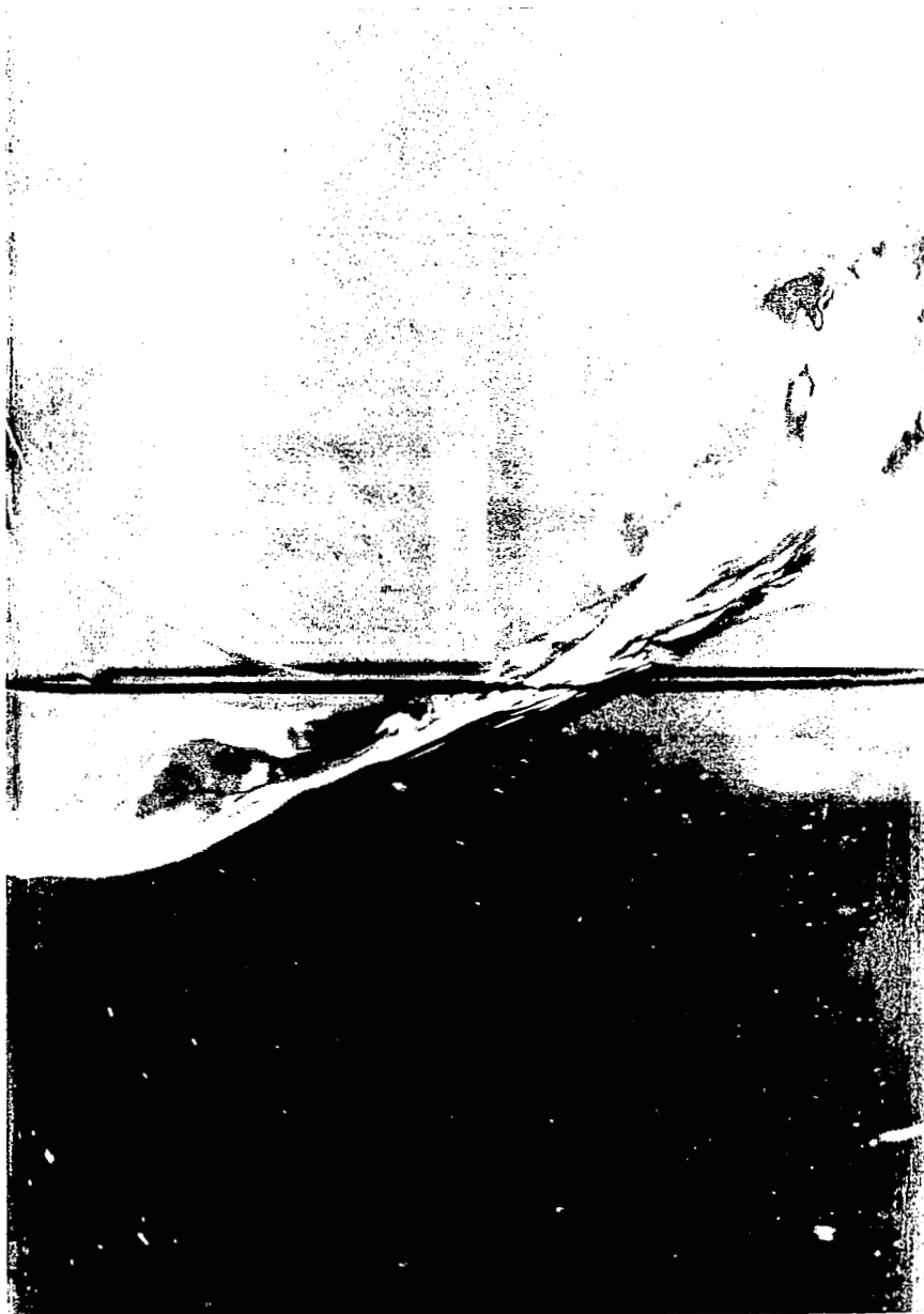
FIGURE I. LARGE AMPLITUDE BREAKING WAVE DURING LATERAL SLOSHING NEAR FIRST MODE RESONANCE
