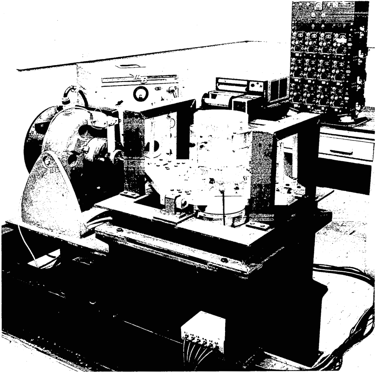
FIGURE 3. EXPERIMENTAL APPARATUS FOR LATERAL SLOSHING
