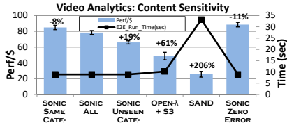
Figure 13: Effect of training SONIC on YouTube video categories similar or dissimilar to test. % over the bars represent the SONIC's (second bar from left) gain over that baseline.
