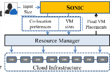
Figure 4: SONIC’s interaction with an existing Resource Manager in the system.
