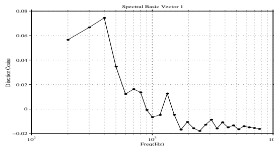
Figure 9: 1st direction cosine of Krumhansl's data set (spectral envelope).
