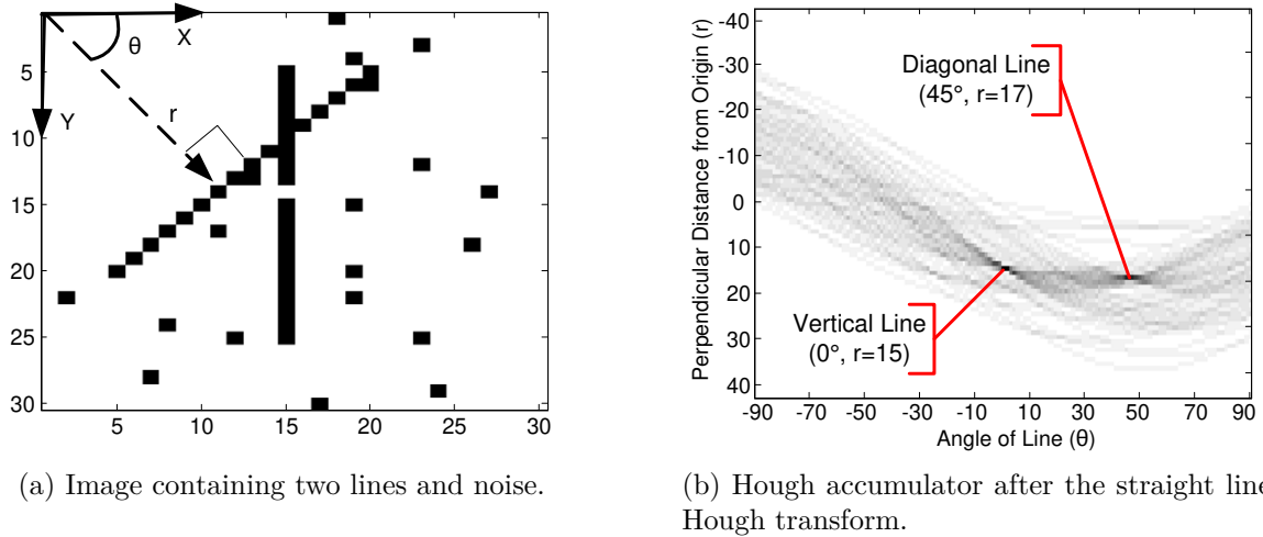
Figure 5.3: Simple example of the Hough transform for overlapping straight lines in noise. The result is two strong local maxima in the Hough accumulator indicating the hypotheses for the two lines.
