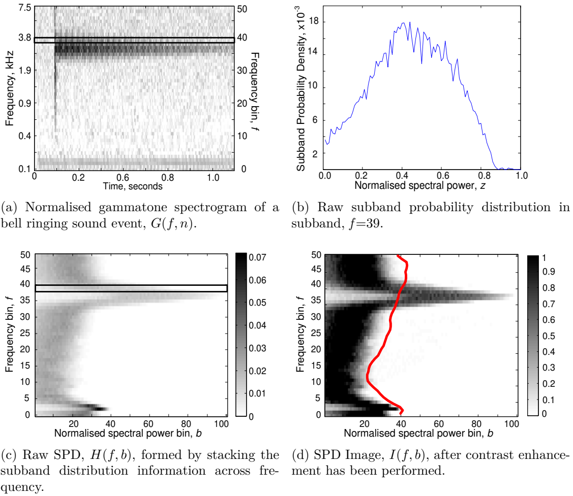
Figure 4.3: Overview of generation of the SPD Image. The probability distribution is taken over each subband, as shown by the example in (b), and are stacked to form the raw SPD in (c). This undergoes contrast enhancement, to give the SPD in (d). The red line in (d) indicates an upper estimate of the noise over the clip. Areas to the right of this line are considered to contain only signal, while the rest is dominated by the noise distribution.
