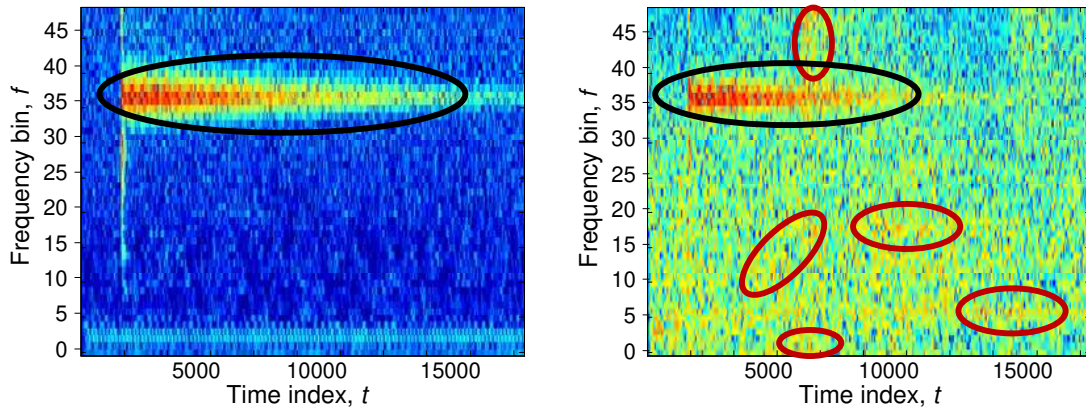
(a) Clean, where it is simple to separate the bell sound from the background noise. (b) Noisy conditions, where regions of noise may be mistaken for signal.
